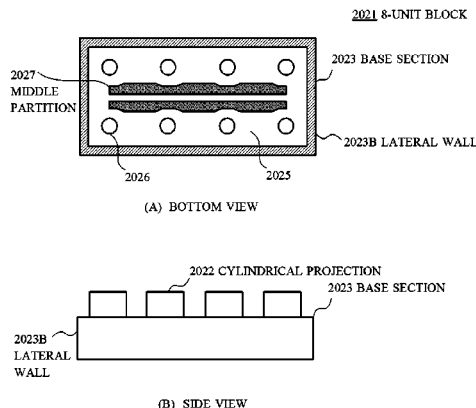
CONFIGURATION OF 8-UNIT BLOCK ACCORDING TO THIRD EMBODIMENT
