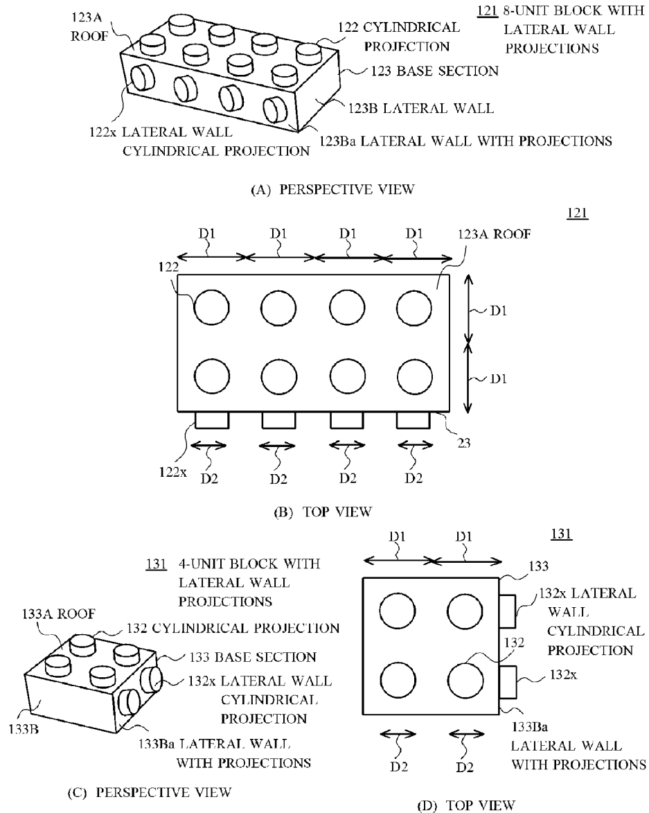
FIG. 12 CONFIGURATION OF BLOCKS WITH LATERAL WALL PROJECTIONS ACCORDING TO FIRST EMBODIMENT
