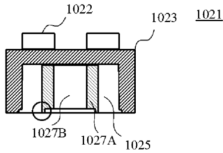
(A) B-B' CROSS-SECTION VIEW
