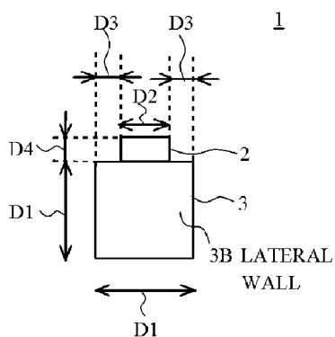
(C) SIDE VIEW
