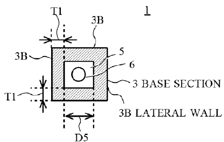
(E) BOTTOM VIEW
