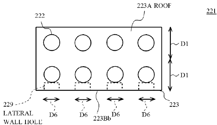
(C) TOP VIEW ILLUSTRATING LATERAL WALL HOLES
