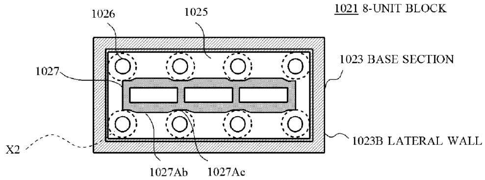
(A) DIAGRAM ILLUSTRATING HOW INTERLOCKING OCCURS
