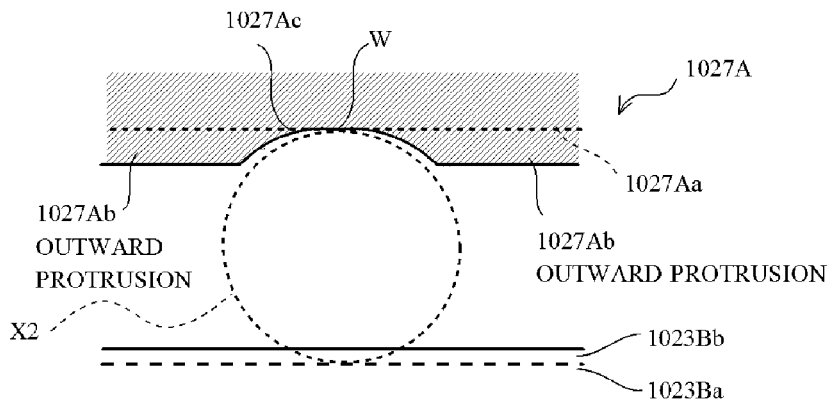
(C) ENLARGED VIEW (2) ILLUSTRATING HOW INTERLOCKING OCCURS
