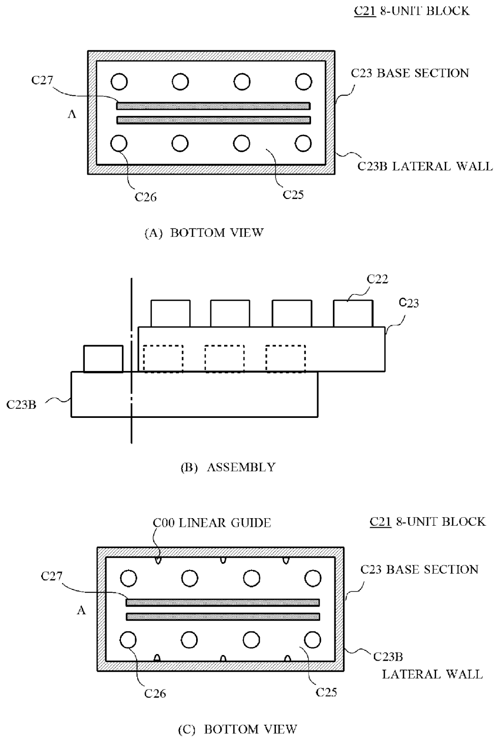
FIG. 19 CONFIGURATION OF CONVENTIONAL 8-UNIT BLOCK
