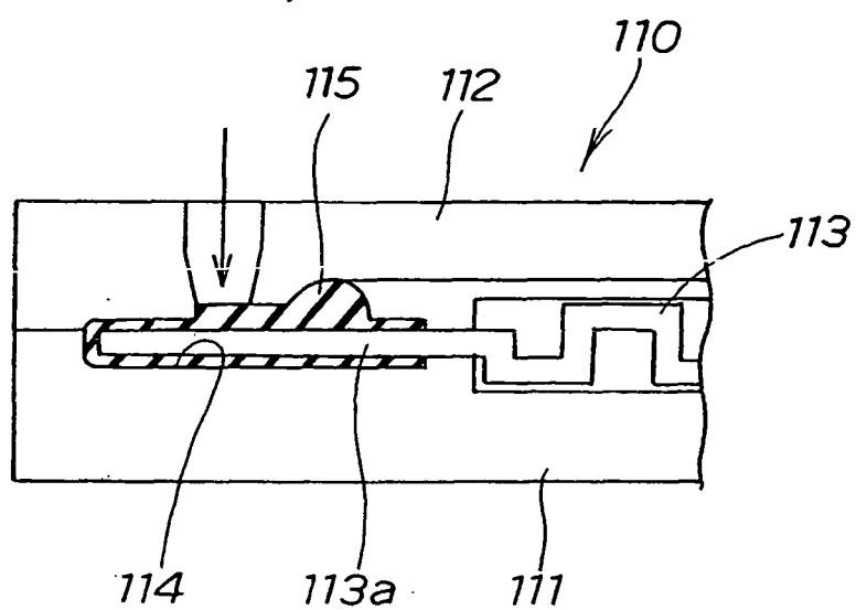
FIG 11 (Prior Art)
