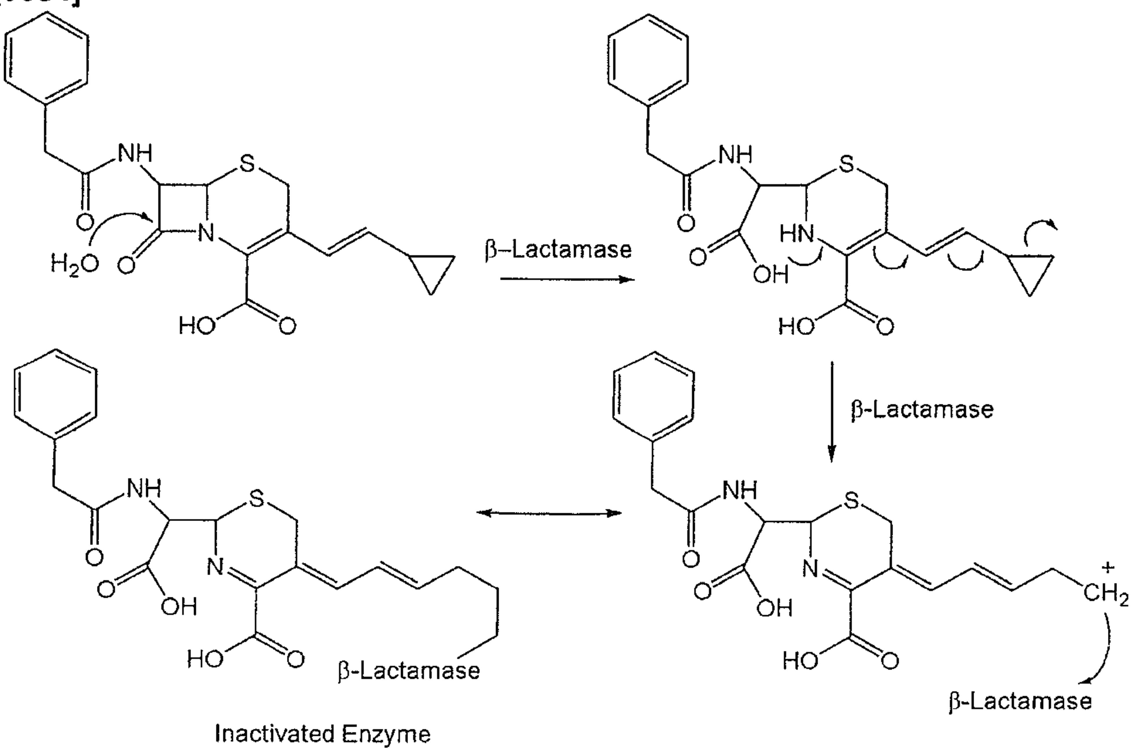
Scheme 4
