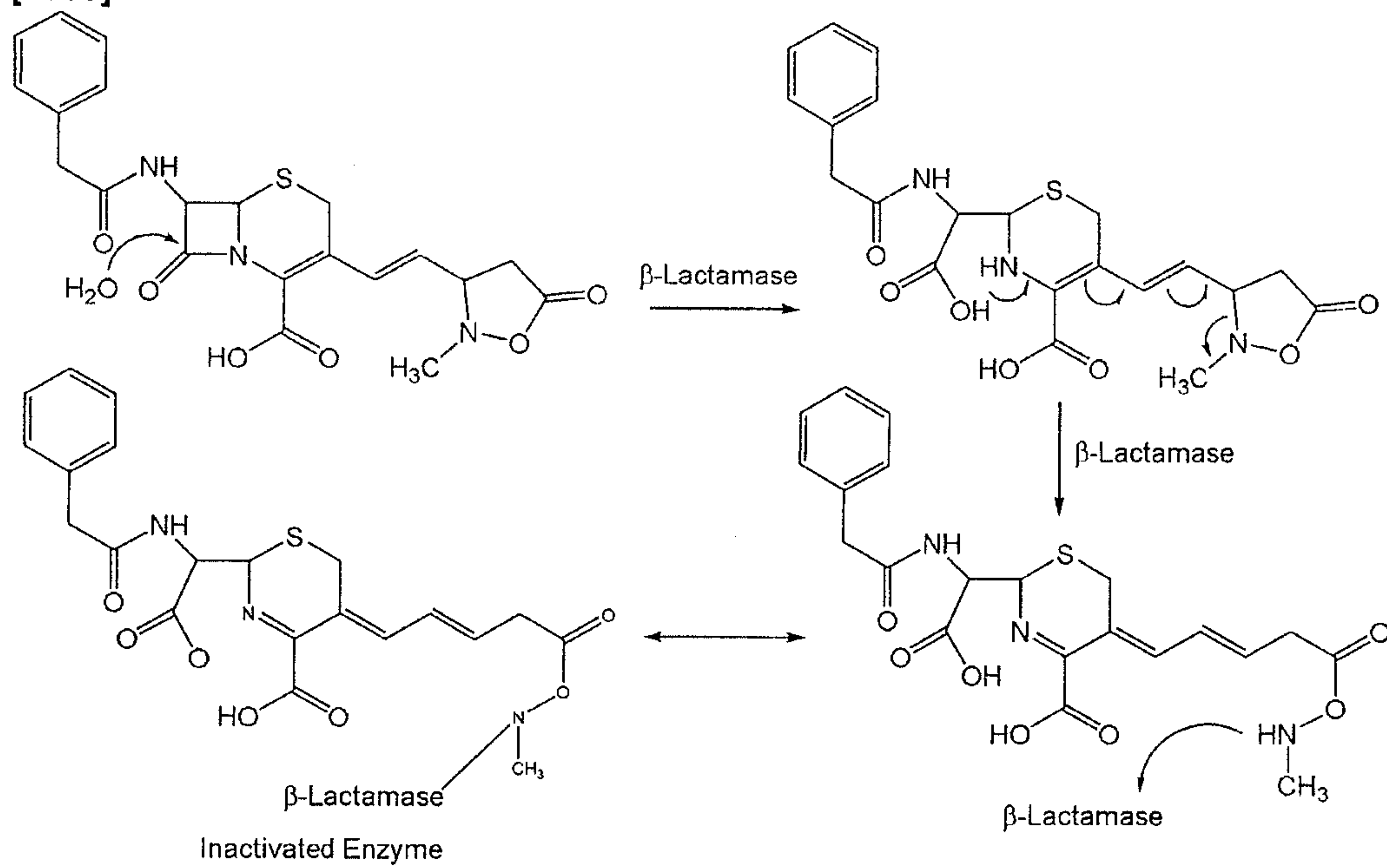
Scheme 3
