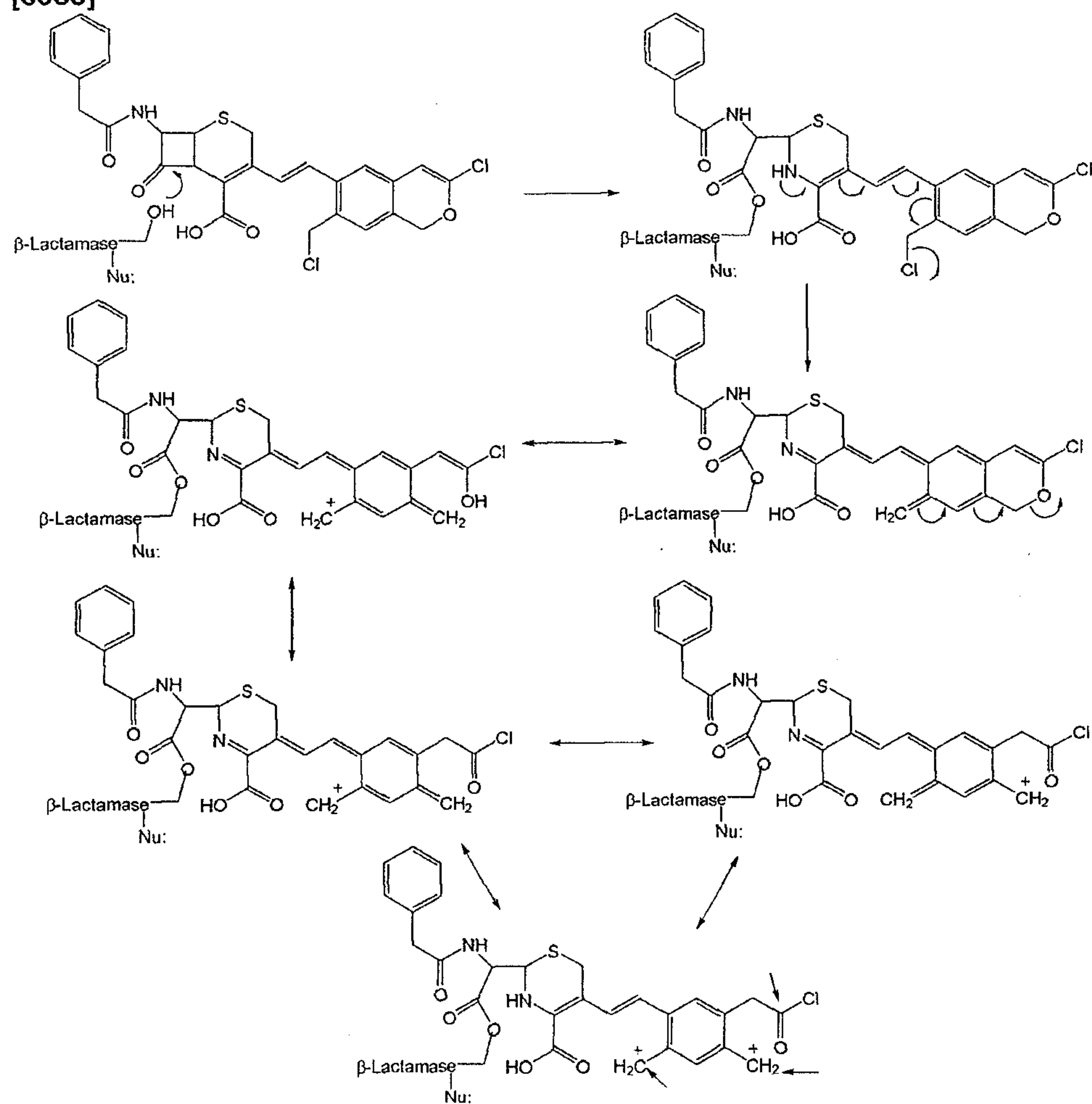
Scheme 5
