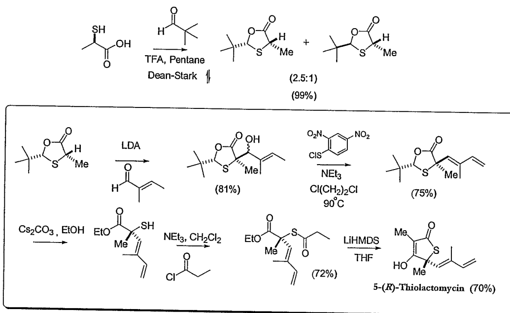
Scheme 1. Asymmetric Synthesis of 5-( R )-Thiolactomycin.
