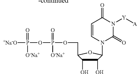
sodium salt of the claimed compound
