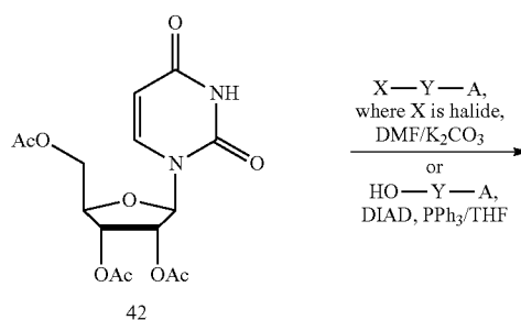
Scheme 1
