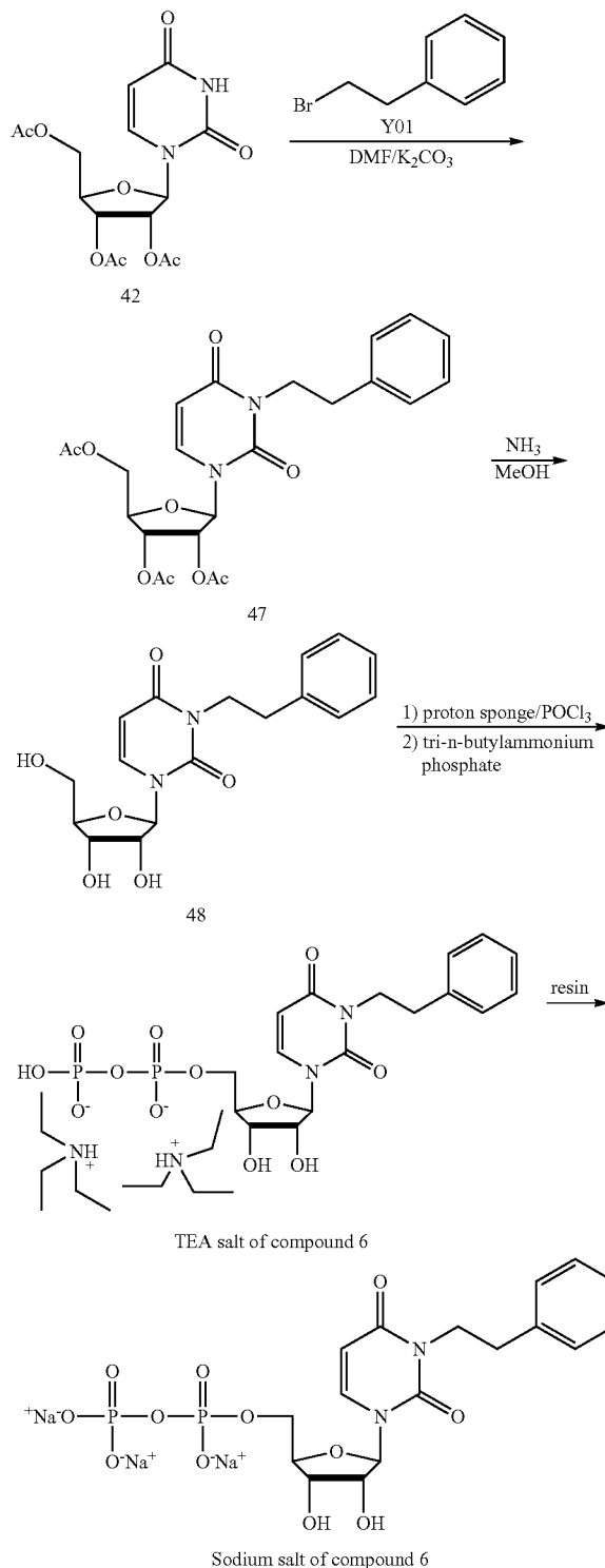
Scheme 2
