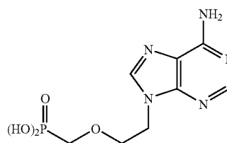
9-[3-(phosphono- methoxy)propyl]adenine (Adefovir)
