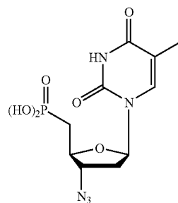
3'-azido-3',5'- dideoxythymidine-5'- phosphonic acid (AZT phosphonate)
