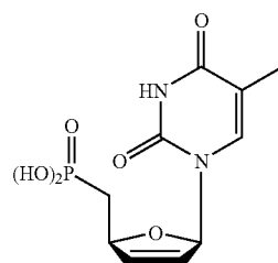
3',5'-dideoxythymidine-2'- ene-5'-phosphonic acid (d4T phosphonate)
