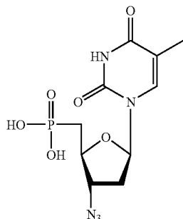
AZT 5'-phosphonate
