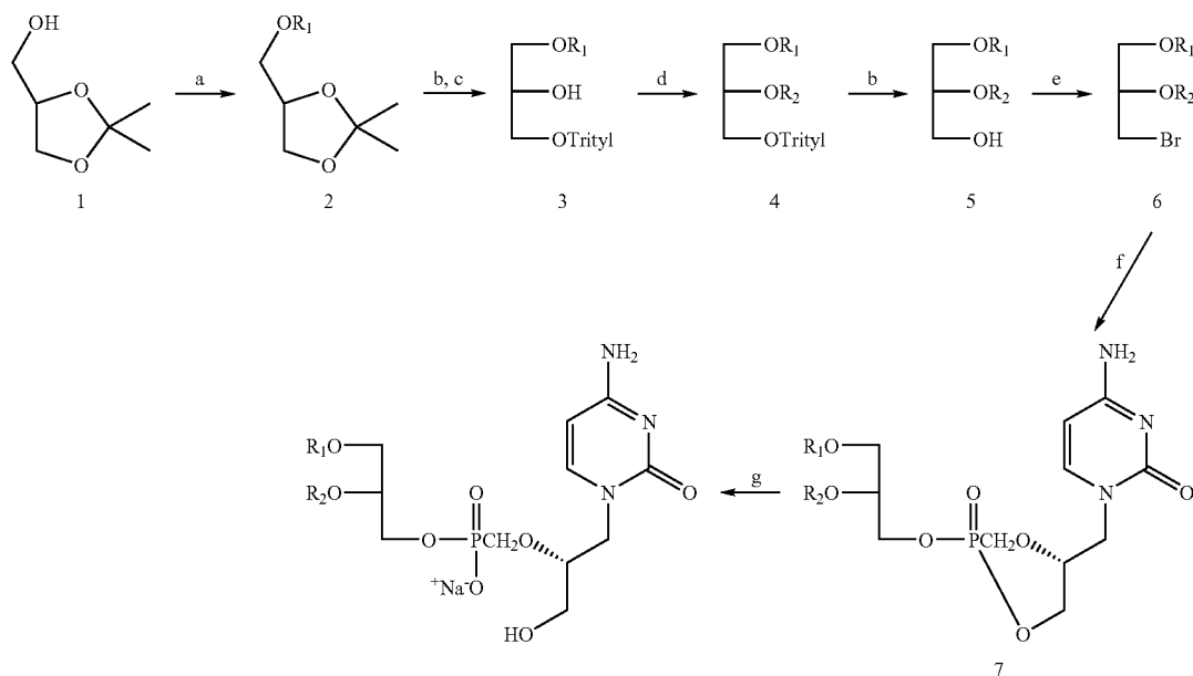
Scheme V
