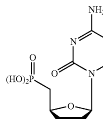
2',3',5'-trideoxycytidine-5'- phosphonic acid (ddC phosphonate)
