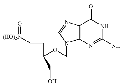
Ganciclovir phosphonate
