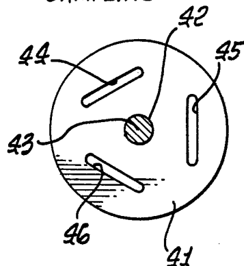
FIG. 4. POSITION: SAMPLING
