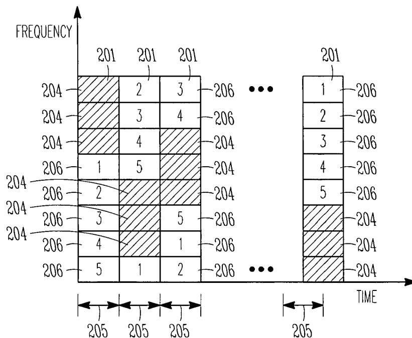
PORTION DOWN LINK SUBFRAME
