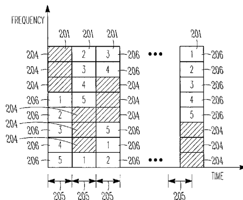
PORTION DOWN LINK SUBFRAME
