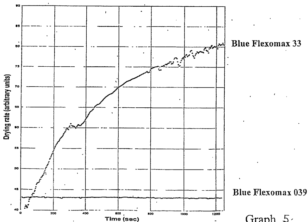
Drying/Resolubility rate of solvent-based laminating inks (PC500L)
