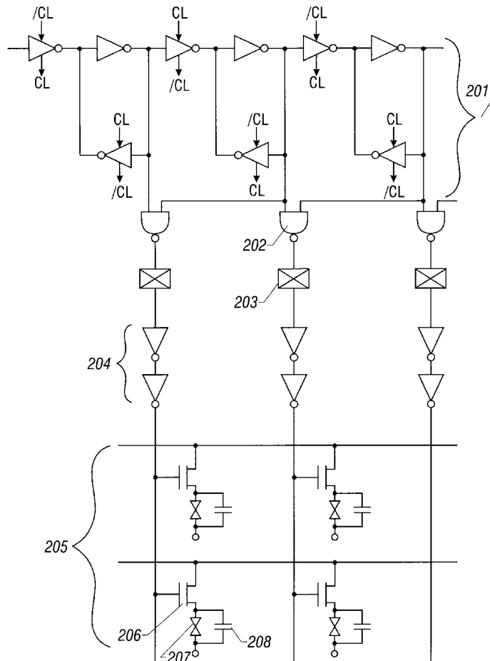
GATE DRIVER CIRCUIT
