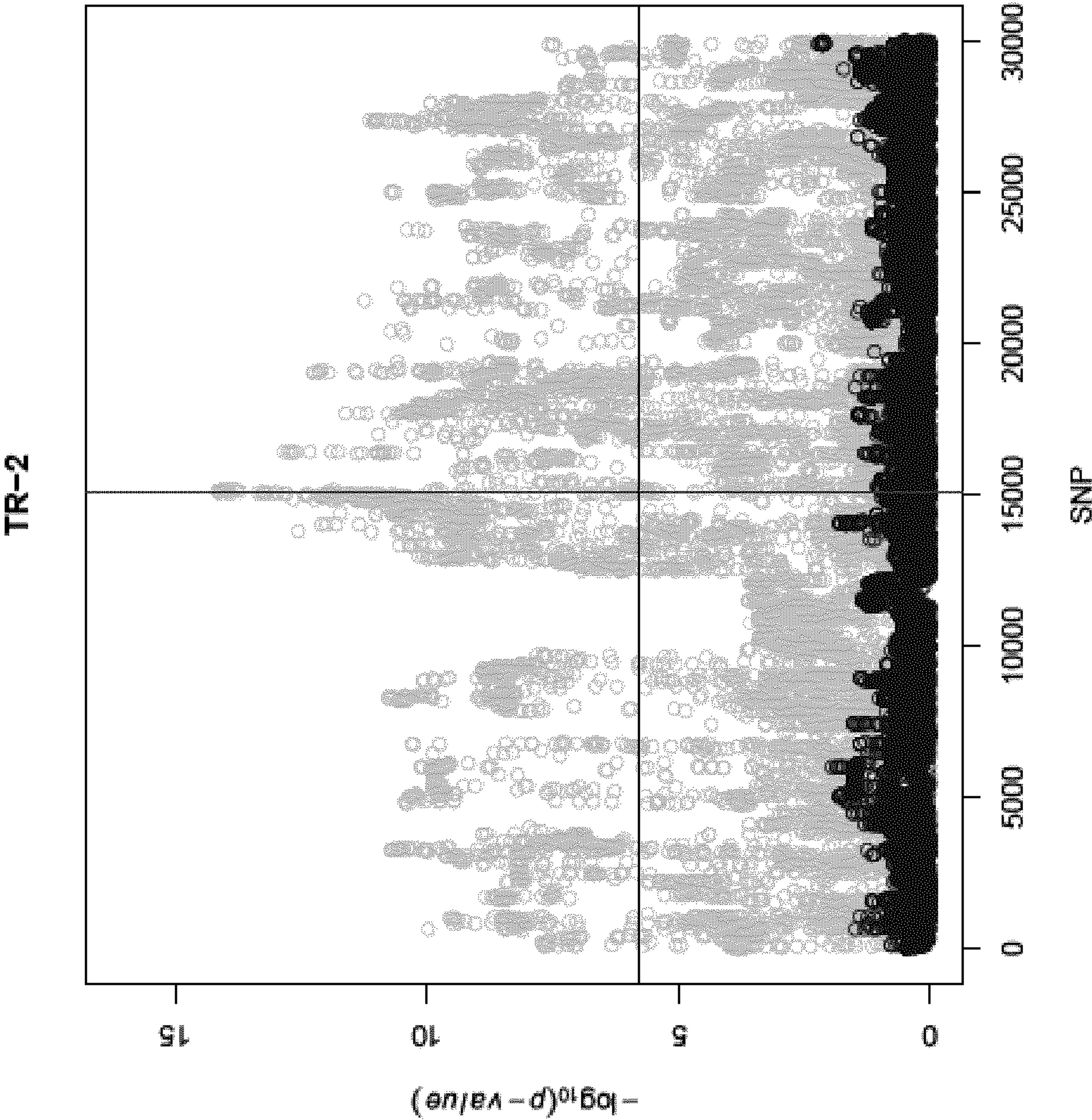
Figure 23, ctd. B. Chr-20.2 MAS12
