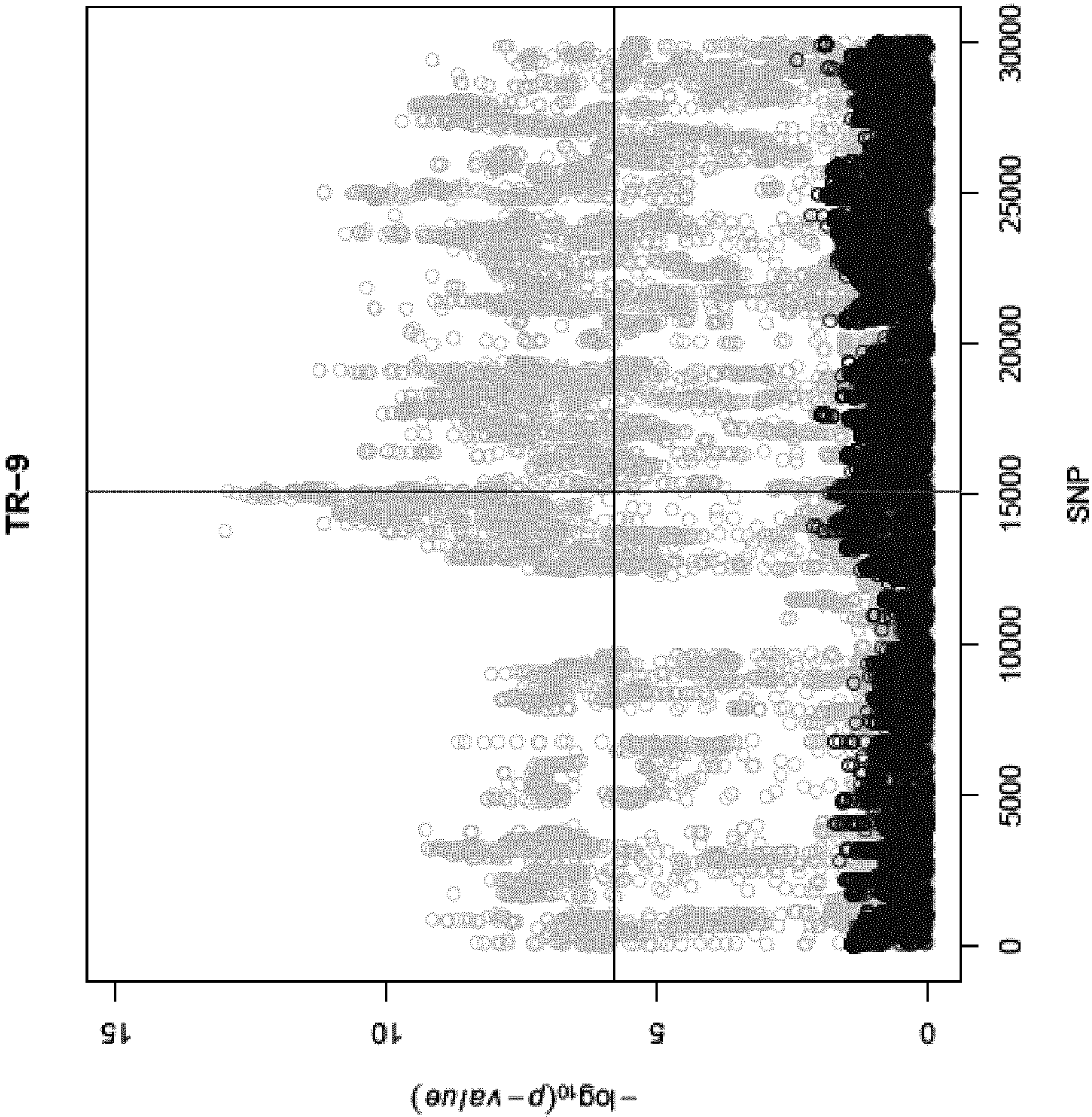
Figure 23, ctd. I. Chr-20.9 SCS-INDEX
