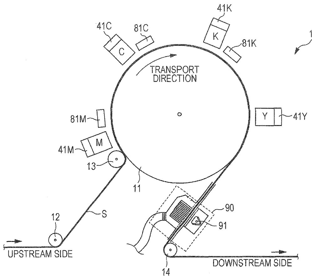
FIG. 1 FIRST EMBODIMENT
