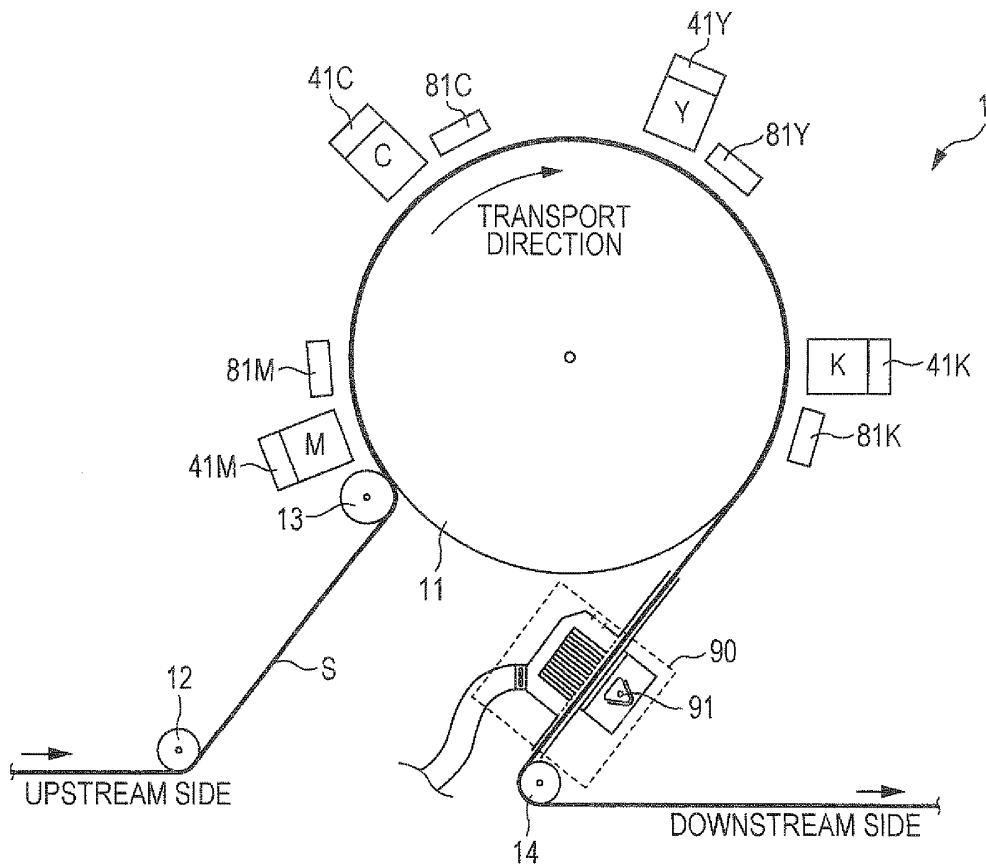
FIG. 4 COMPARATIVE EXAMPLE
