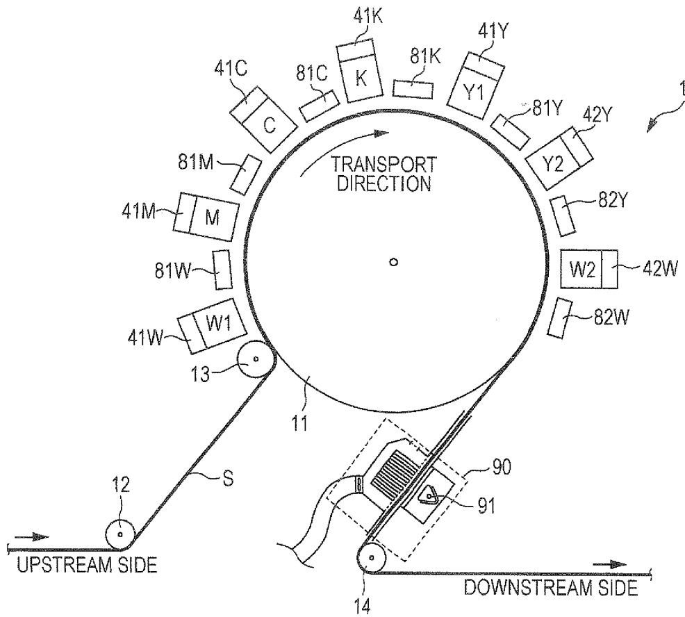
FIG. 8 FOURTH EMBODIMENT
