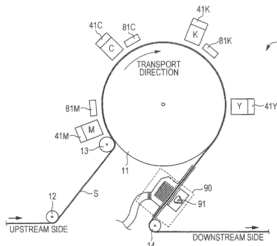
FIG. 1 FIRST EMBODIMENT
