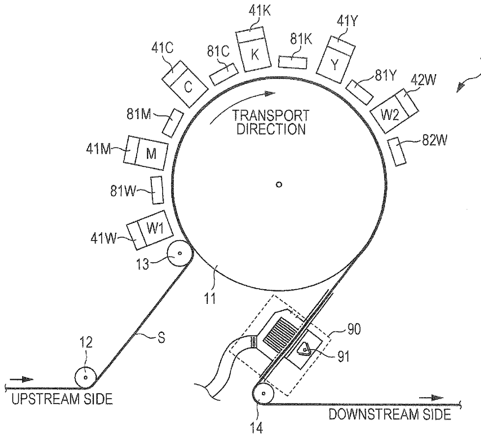
FIG. 6 THIRD EMBODIMENT
