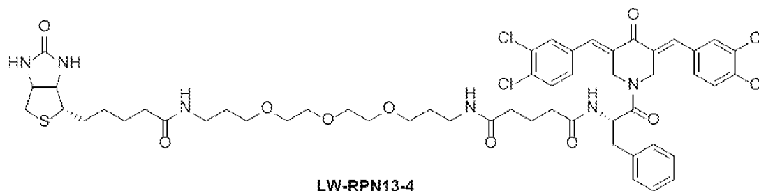
Scheme 1. Exemplary synthesis of LW-RPN13-4
