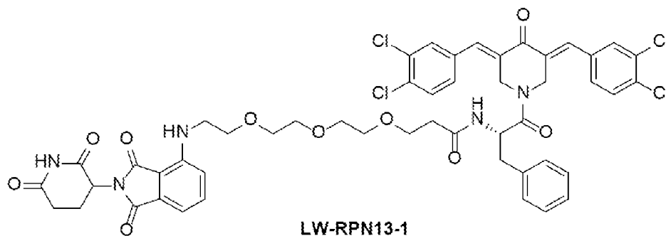
Scheme 2. Exemplary synthesis of LW-RPN13-1
