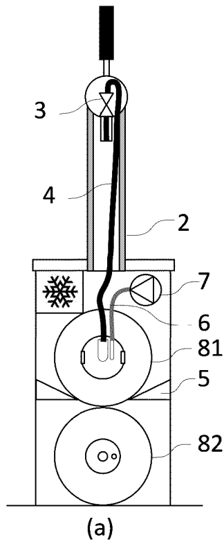
FIG. 1 (PRIOR ART)
