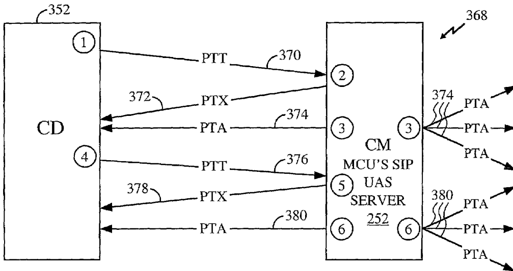
FIG. 12 MEDIA SIGNALING MESSAGE SEQUENCE (PTT)
