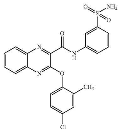
2-(4-chloro-2-methylphenoxy)-N-(3-sulfamoylphenyl)quinoline-3-carboxamide
