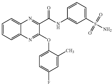
3-(4-fluoro-2-methylphenoxy)-N-(3-sulfamoylphenyl)quinoxaline-2-carboxamide
