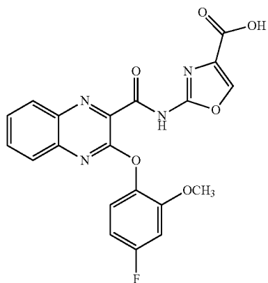
2-(3-(4-fluoro-2-methoxyphenoxy)quinoxaline-2-carboxamido)oxazole-4-carboxylic acid
