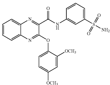
3-(2,4-dimethoxyphenoxy)-N-(3-sulfamoylphenyl)quinoxaline-2-carboxamide
