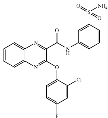
2-(2-chloro-4-fluorophenoxy)-N-(3-sulfamoylphenyl)quinoline-3-carboxamide
