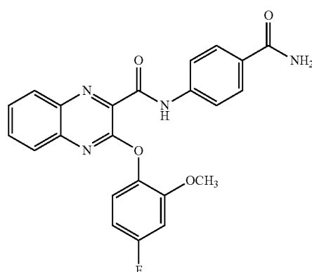
N-(4-carbamoylphenyl)-3-(4-fluoro-2-methoxyphenoxy)quinoxaline-2-carboxamide
