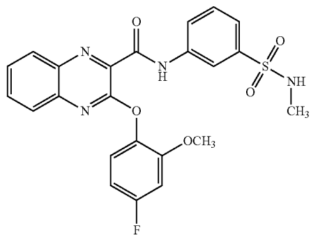
3-(4-fluoro-2-methylphenoxy)-N-(N-methylsulfamoyl)phenyl)quinoxaline-2-carboxamide
