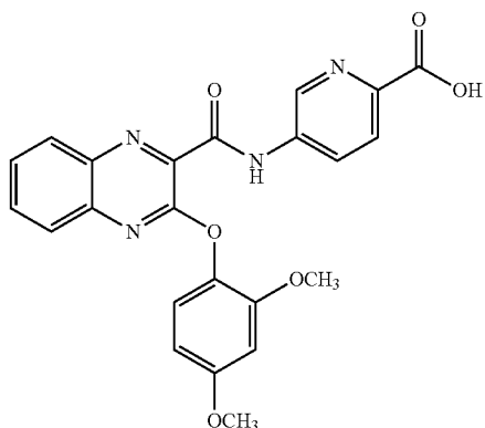
5-(3-(2,4-dimethoxyphenoxy)quinoxaline-2-carboxamido)picolinic acid
