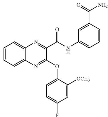
N-(3-carbamoylphenyl)-3-(4-fluoro-2-methoxyphenoxy)quinoxaline-2-carboxamide
