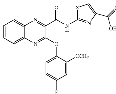
2-(3-(4-fluoro-2-methoxyphenoxy)quinoxaline-2-carboxamido)thiazole-4-carboxylic acid
