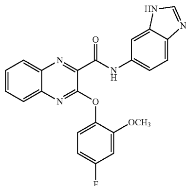
N-(1H-benzod[imidazol-6-yl]-3-(4-fluoro-2-methoxyphenoxy)quinoxaline-2-carboxamide
