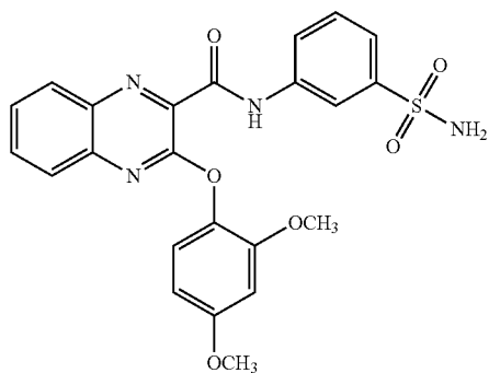
3-(2,4-dimethoxyphenoxy)-N-(3-sulfamoylphenyl)quinoxaline-2-carboxamide
