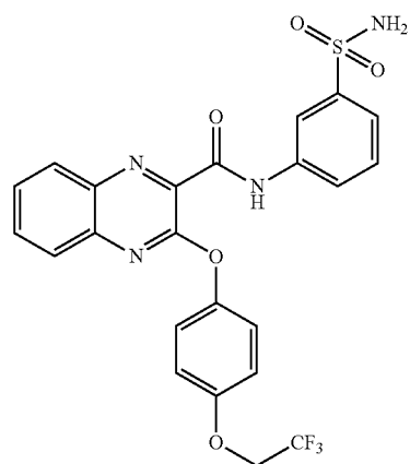
N-(3-sulfamoylphenyl)-2-(4-(2,2,2-trifluoroethoxy)phenoxy)quinoline-3-carboxamide
