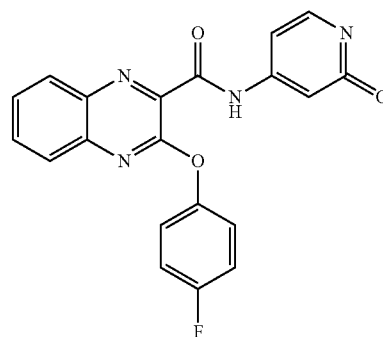
3-(4-fluorophenoxy)-N-(2-oxo-1,2-dihydropyridin-4-yl)quinoxaline-2-carboxamide
