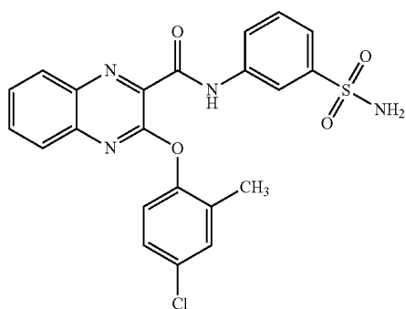
3-(4-chloro-2-methylphenoxy)-N-(3-sulfamoylphenyl)quinoxaline-2-carboxamide
