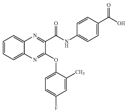
4-(2-(4-fluoro-2-methylphenoxy)quinolin-3-yl)benzoic acid
