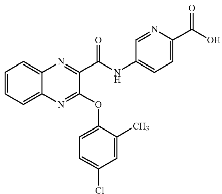
5-(3-(4-chloro-2-methylphenoxy)quinoxaline-2-carboxamido)picolinic acid
