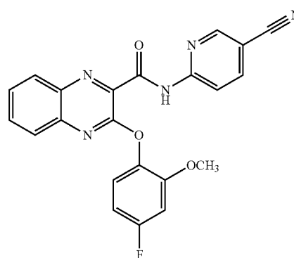
N-(5-cyanopyridin-2-yl)-3-(4-fluoro-2-methoxyphenoxy)quinoxaline-2-carboxamide
