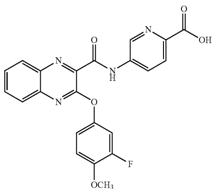
5-(3-(3-fluoro-4-methoxyphenoxy)quinoxaline-2-carboxamido)picolinic acid
