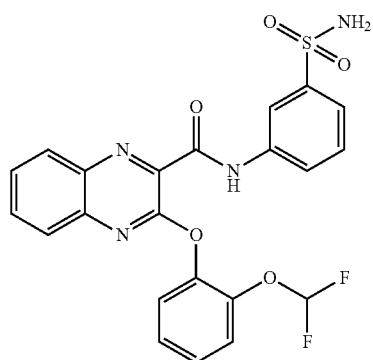
2-(2-(difluoromethoxy)phenoxy)-N-(3-sulfamoylphenyl)quinoline-3-carboxamide
