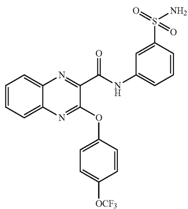
N-(3-sulfamoylphenyl)-2-(4-trifluoromethoxyphenoxy)quinoline-3-carboxamide
