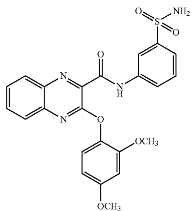
2-(2,4-dimethoxyphenoxy)-N-(3-sulfamoylphenyl)quinoline-3-carboxamide
