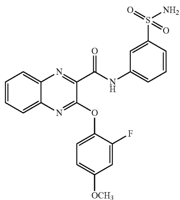
2-(2-fluoro-4-methoxyphenoxy)-N-(3-sulfamoylphenyl)quinoline-3-carboxamide
