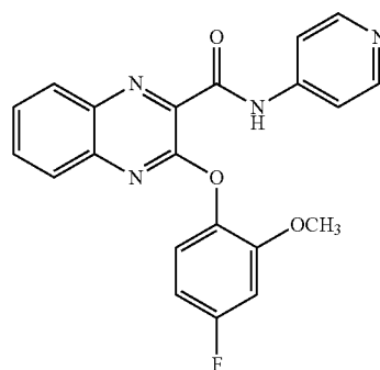
3-(4-fluoro-2-methoxyphenoxy)-N-(pyridin-4-yl)quinoxaline-2-carboxamide
