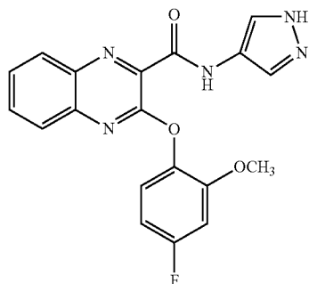
3-(4-fluoro-2-methoxyphenoxy)-N-(1H-pyrazol-4-yl)quinoxaline-2-carboxamide
