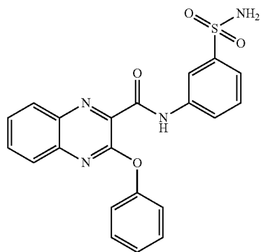
2-phenoxy)-N-(3-sulfamoylphenyl)quinoline-3-carboxamide
