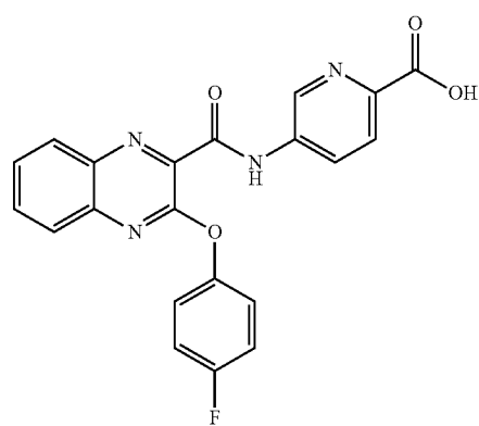
5-(3-(4-(fluorophenoxy)quinoxaline-2-carboxamido)picolinic acid
