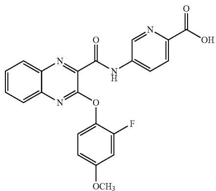
5-(3-(2-(fluoro-4-methoxyphenoxy)quinoxaline-2-carboxamido)picolinic acid
