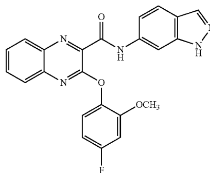
3-(4-fluoro-2-methoxyphenoxy)-N-(1H-indazol-6-yl)quinoxaline-2-carboxamide
