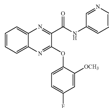
3-(4-fluoro-2-methoxyphenoxy)-N-(pyridin-3-yl)quinoxaline-2-carboxamide
