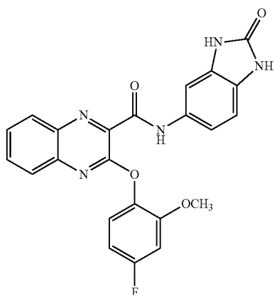
3-(4-fluoro-2-methoxyphenoxy)-N-(2-oxo-2,3-dihydro-1H-benzo[d]imidazol-5-yl)quinoxaline-2-carboxamide
