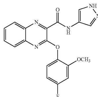
3-(4-fluoro-2-methoxyphenoxy)-N-(1H-pyrazol-4-yl)quinoxaline-2-carboxamide
