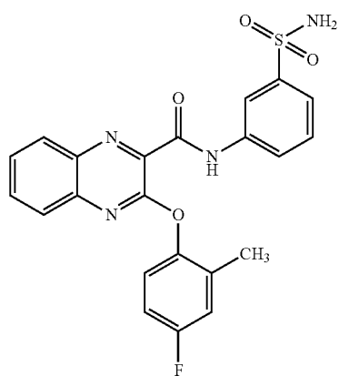
2-(4-fluoro-2-methylphenoxy)-N-(3-sulfamoylphenyl)quinoline-3-carboxamide
