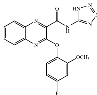
3-(4-fluoro-2-methoxyphenoxy)-N-(1H-tetrazol-5-yl)quinoxaline-2-carboxamide
