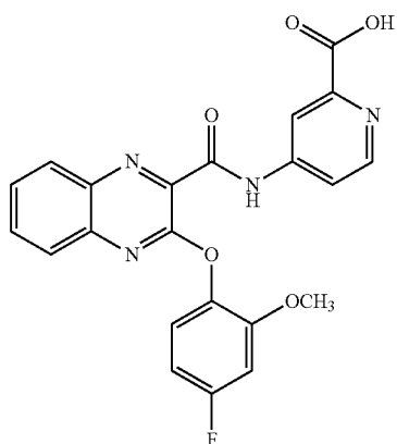
4-(3-(4-fluoro-2-methoxyphenoxy)quinoxaline-2-carboxamido)picolinic acid
