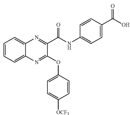
4-(3-(4-(trifluoromethoxy)phenoxy)quinoxaline-2-carboxamido)benzoic acid
