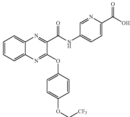
5-(3-(4-(2,2,2-trifluoroethoxy)phenoxy)quinoxaline-2-carboxamido)picolinic acid
