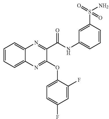
2-(2,4-difluorophenoxy)-N-(3-sulfamoylphenyl)quinoline-3-carboxamide
