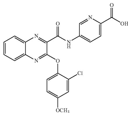
5-(3-(2-chloro-4-methoxyphenoxy)quinoxaline-2-carboxamido)picolinic acid
