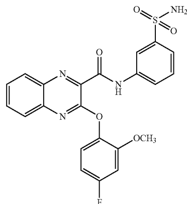
2-(4-fluoro-2-methoxyphenoxy)-N-(3-sulfamoylphenyl)quinoline-3-carboxamide
