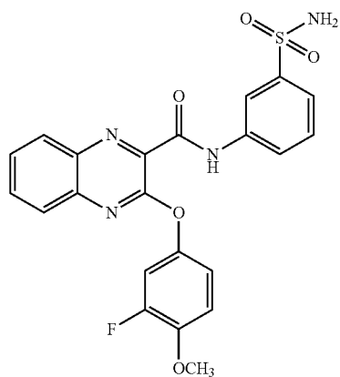
2-(3-fluoro-4-methoxyphenoxy)-N-(3-sulfamoylphenyl)quinoline-3-carboxamide
