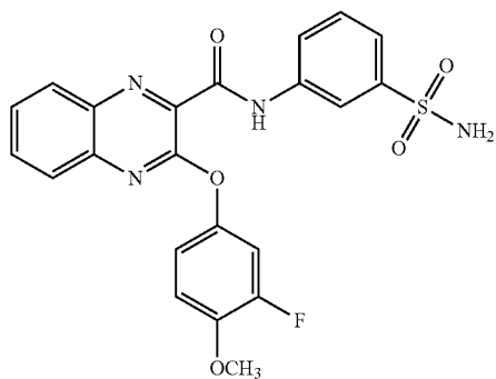
3-(3-fluoro-4-methoxyphenoxy)-N-(3-sulfamoylphenyl)quinoxaline-2-carboxamide
