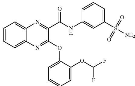
3-(2-(difluoromethoxy)phenoxy)-N-(3-sulfamoylphenyl)quinoxaline-2-carboxamide
