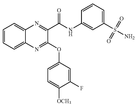
3-(3-fluoro-4-methoxyphenoxy)-N-(3-sulfamoylphenyl)quinoxaline-2-carboxamide
