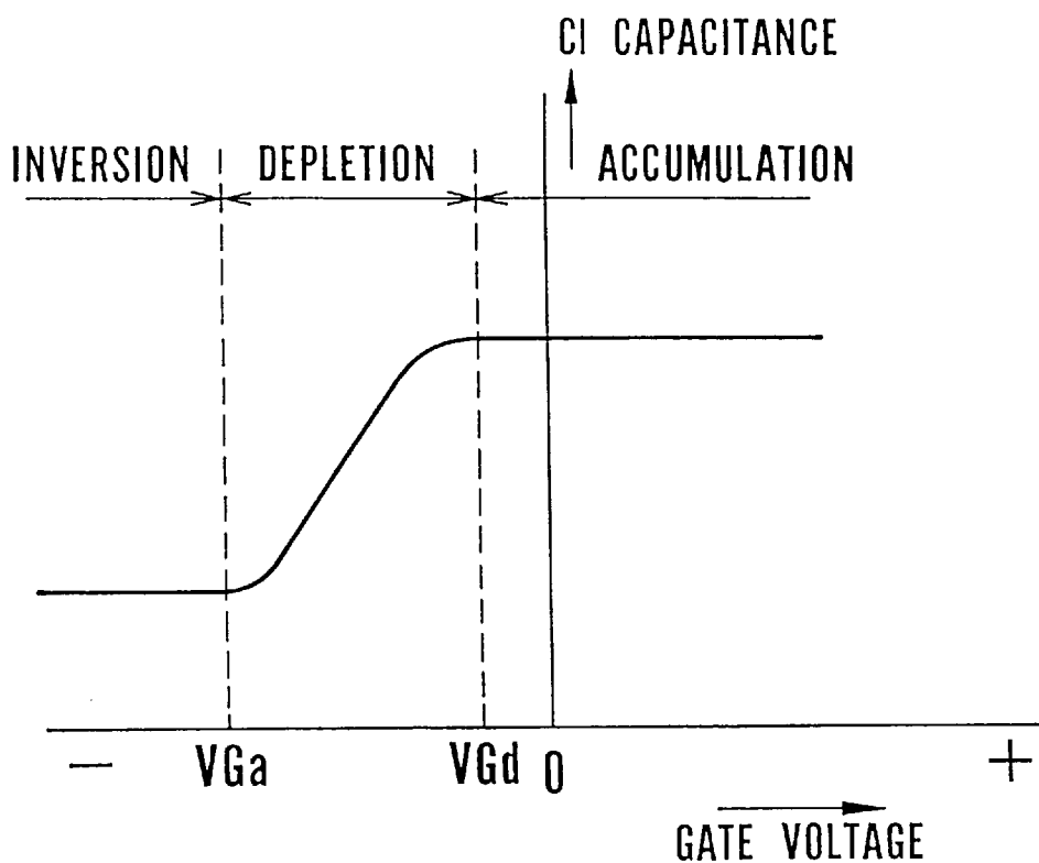
FIG. 2 PRIOR ART
