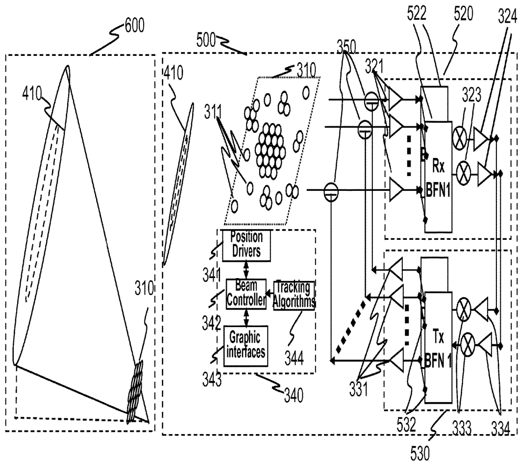
A multi-beam dish antenna with defocused array feeds beam shaping via element positioning Figure 6
