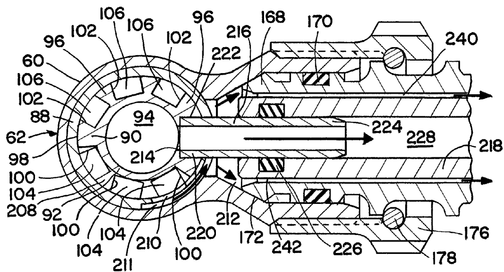
SECTION N - N
