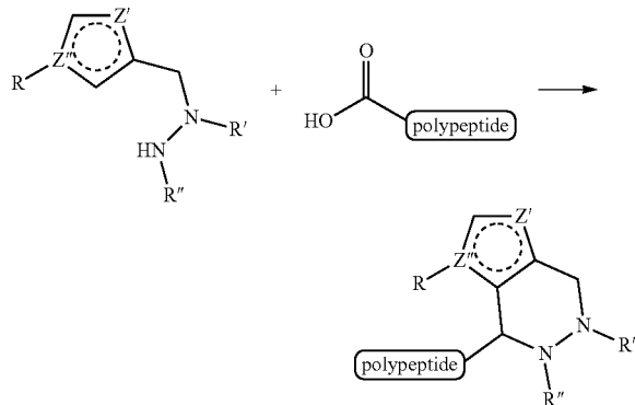
General Reaction Scheme A
