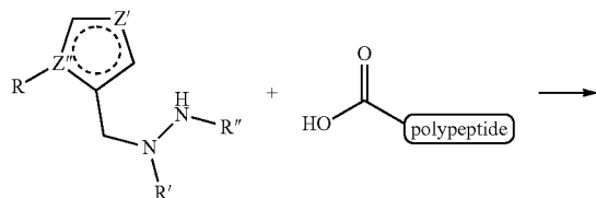
General Reaction Scheme B
