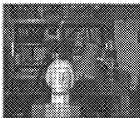
Master image
