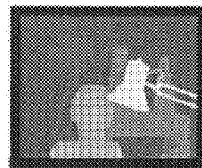
Disparity map
