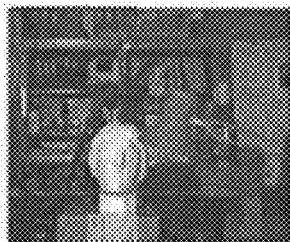
Slave image
