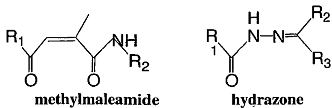
Figure D-2-2: Acid-labile linkers.
