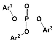
[Chemical Formula 1]
