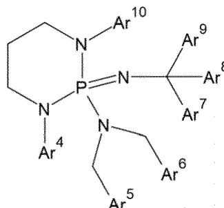
[Chemical Formula 2]
