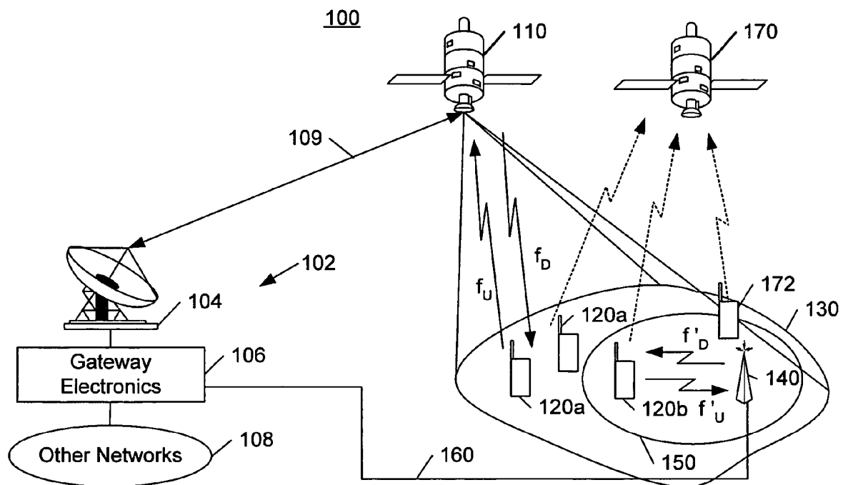
Figure 1 (Prior Art)
