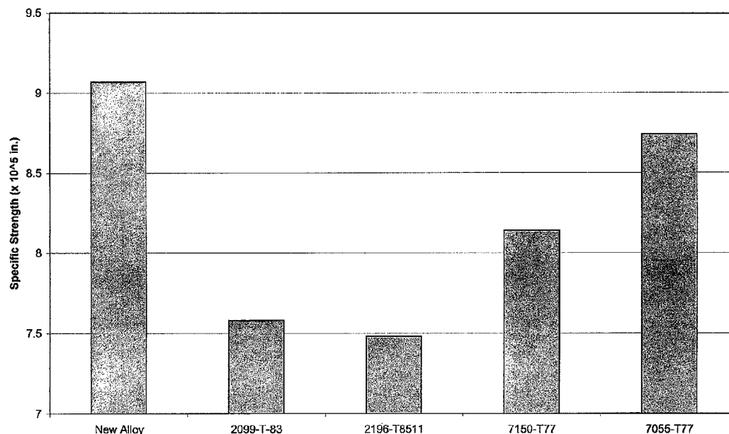
Specific Strength of Alloys (typical)
