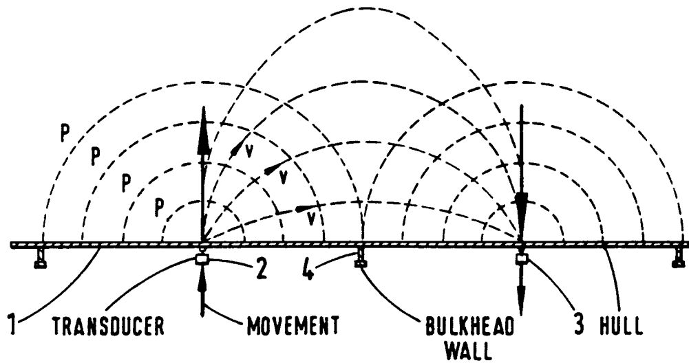
Fig. 1 PRESSURE AND VELOCITY DIPOLES
