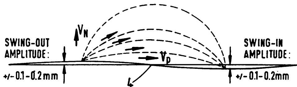
Fig. 2 VELOCITY VECTORS
