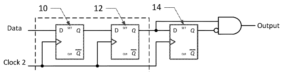
FIG. 2 (Prior Art)
