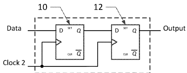
FIG. 1 (Prior Art)
