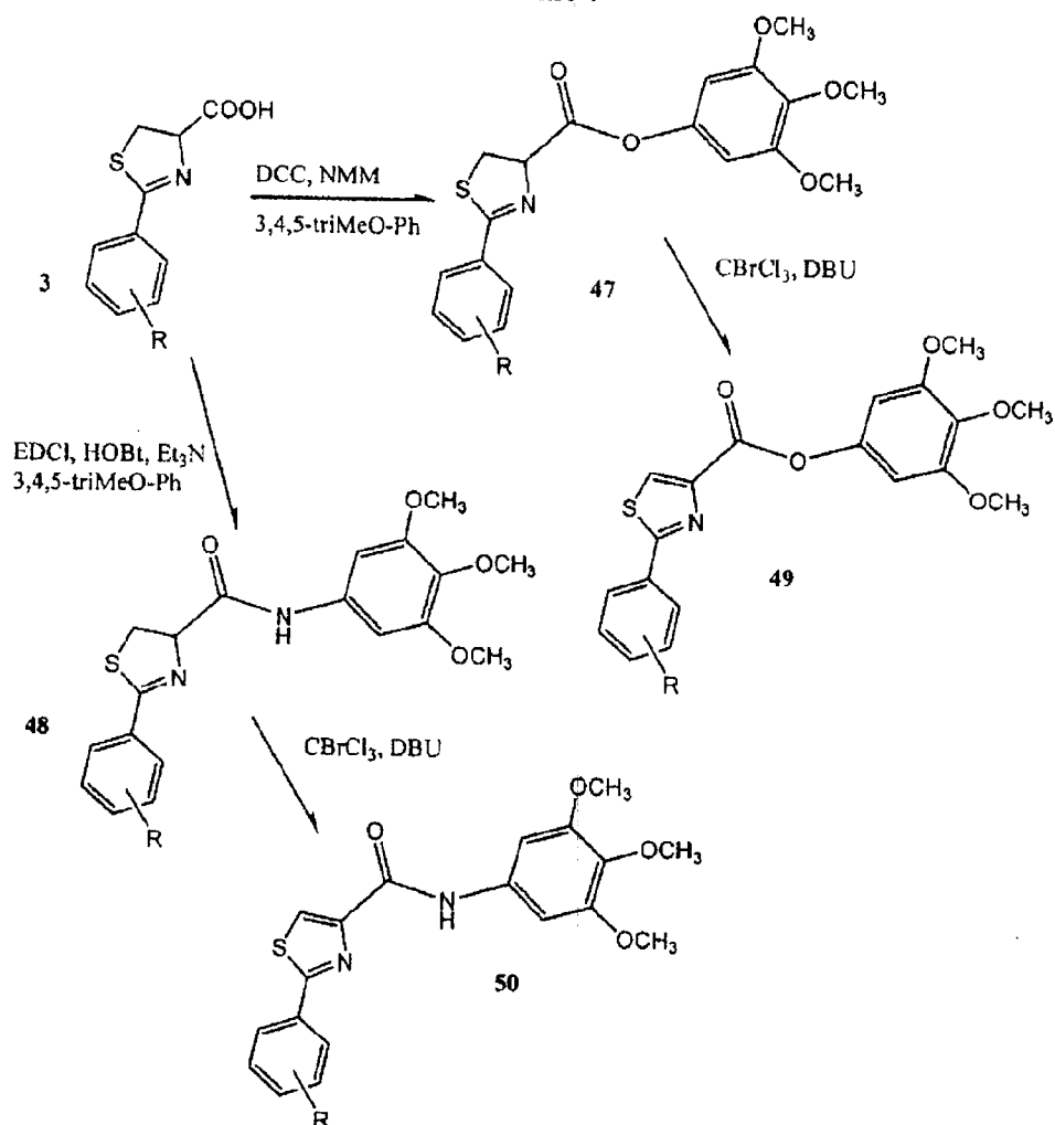
Scheme 7
