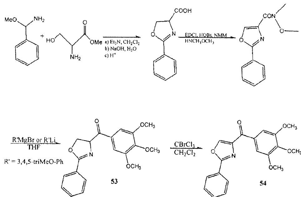
Scheme 8B
