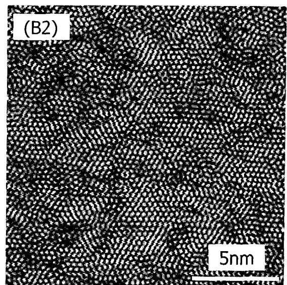
CAAC-OS film (inverse Fourier transform image)
