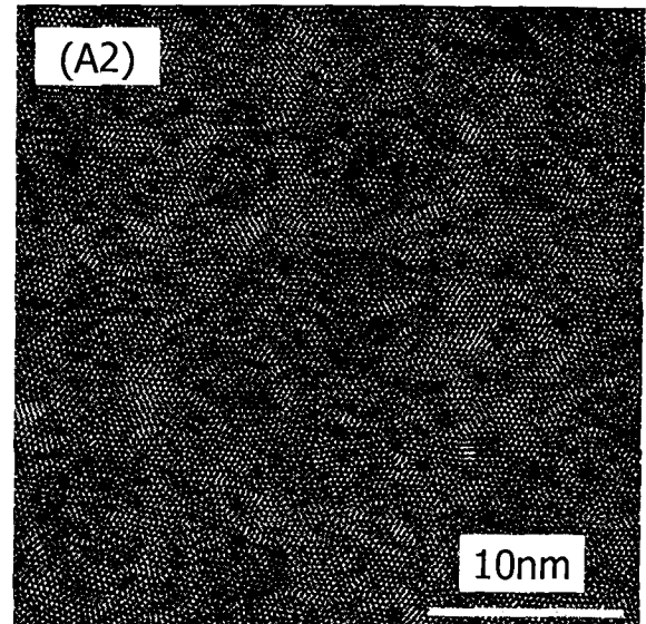
CAAC-OS film (inverse Fourier transform image)
