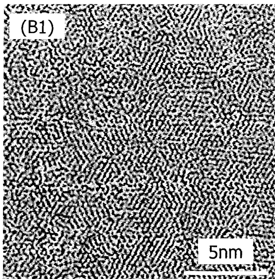
CAAC-OS film (high-resolution plan-view TEM image)
