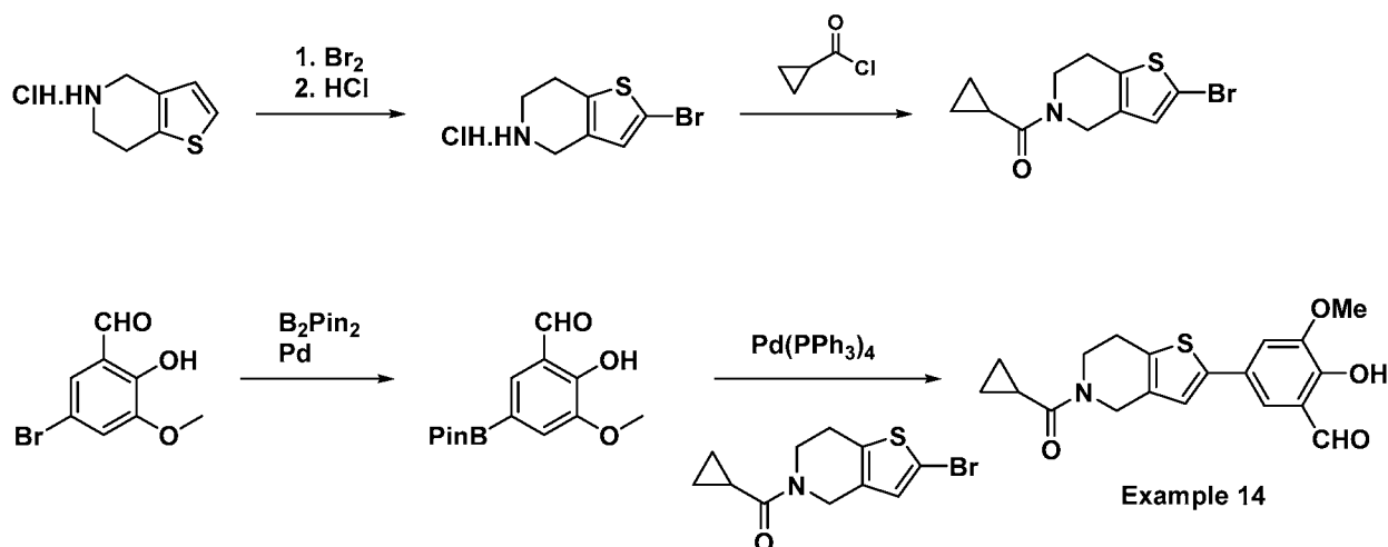
Example 14: 5-(5-(cyclopropanecarbonyl)-4,5,6,7-tetrahydrothieno[3,2-c]pyridin-2-yl)-2-hydroxy-3-methoxybenzaldehyde
