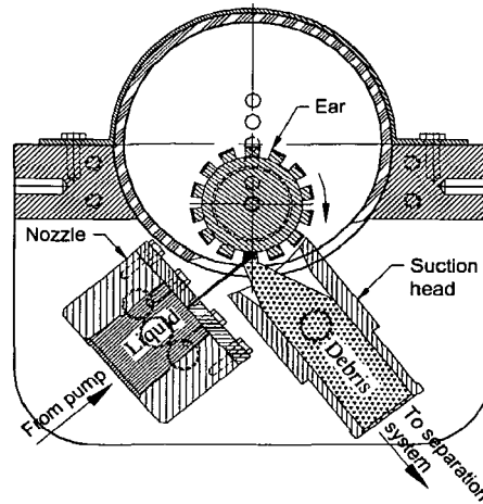
Fig. 3 Embryos excision by a flat "sheet" of water testing device.
