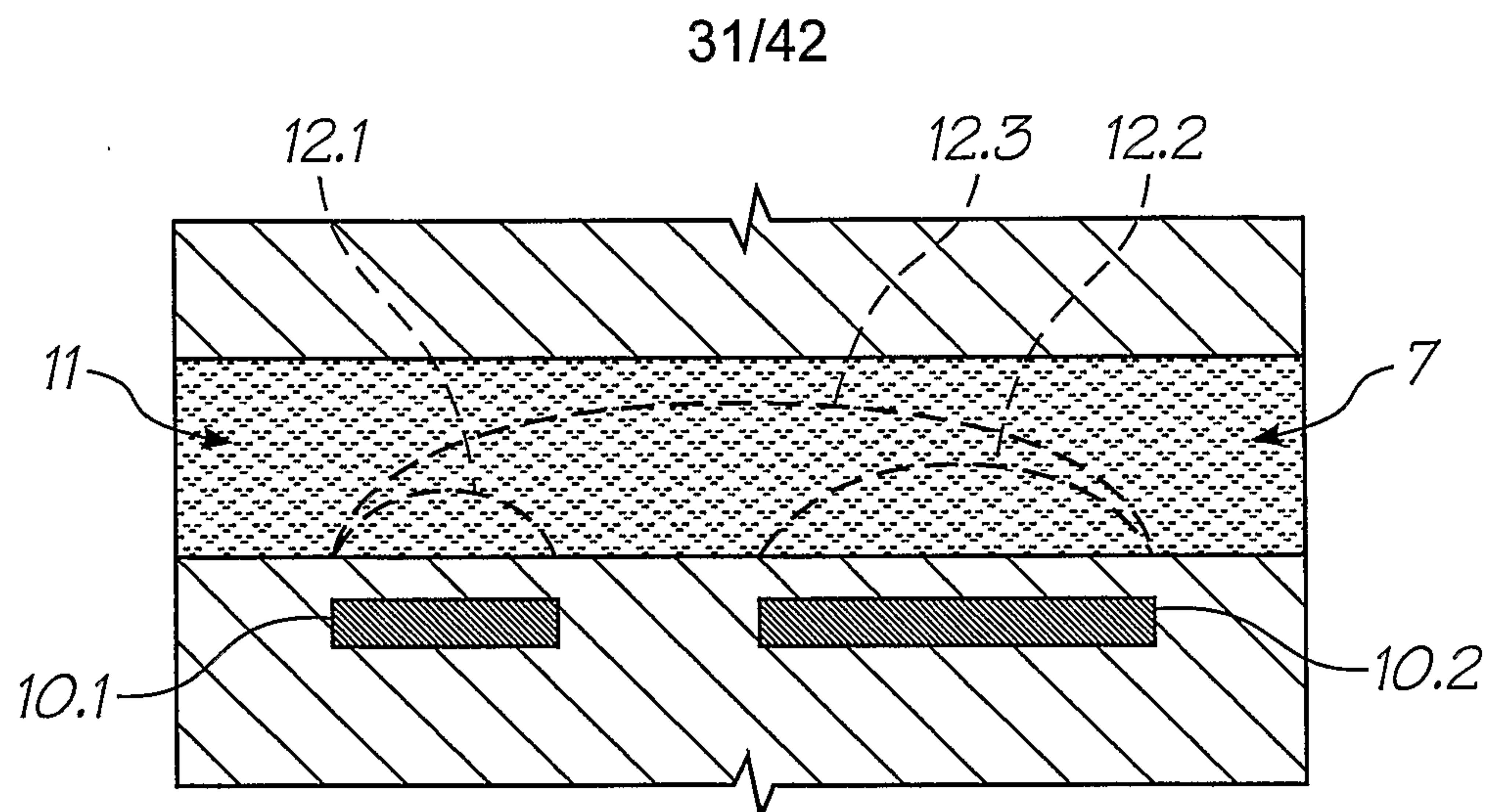
FIG. 52 (PRIOR ART)
