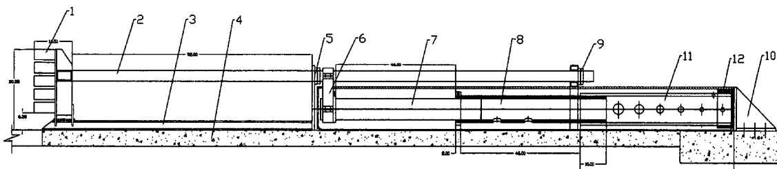
SIDE ELEVATION CROSS SECTION AT NORMAL POSITION
