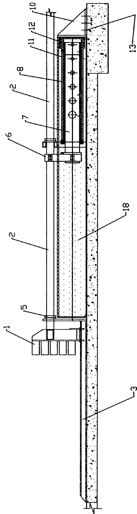
FIG 2. SIDE ELEVATION CROSS SECTION AT FULLY RETRACTED WHEN HIT BY HEAVY VEHICLE
