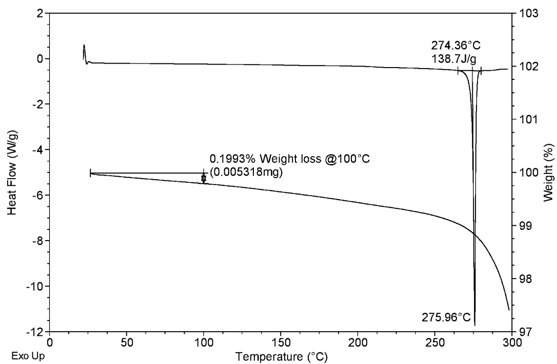
FIG. 2: DSC trace of 6-fluoro-5-[4-[(5-fluoro-2-methyl-3-oxo-4H-quinoxalin-6-yl)methyl]piperazin-1-yl]-N-methyl-pyridine-2-carboxamide Form B
