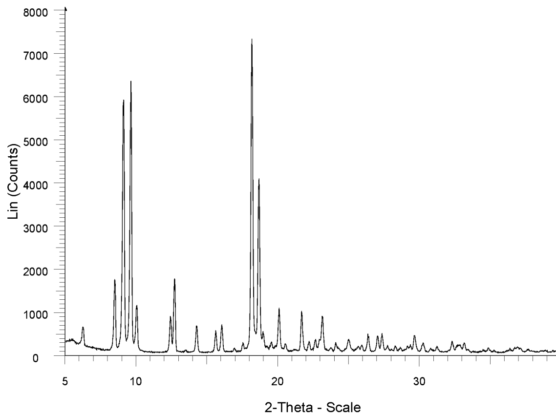
FIG. 1: XRPD diffractogram of 6-fluoro-5-[4-[(5-fluoro-2-methyl-3-oxo-4H-quinoxalin-6-yl)methyl]piperazin-1-yl]-N-methyl-pyridine-2-carboxamide Form B
