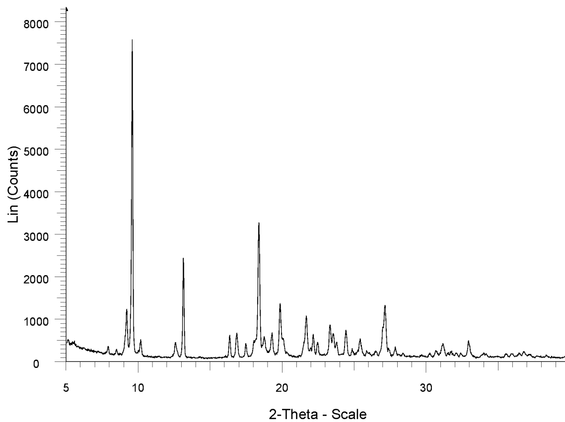
FIG. 3 : XRPD diffractogram of 6-fluoro-5-[4-[(5-fluoro-2-methyl-3-oxo-4H-quinoxalin-6-yl)methyl]piperazin-1-yl]-N-methyl-pyridine-2-carboxamide Form D
