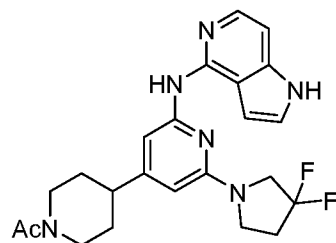
Compound 119
