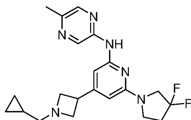
Compound 167
