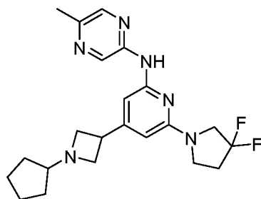
Compound 169
