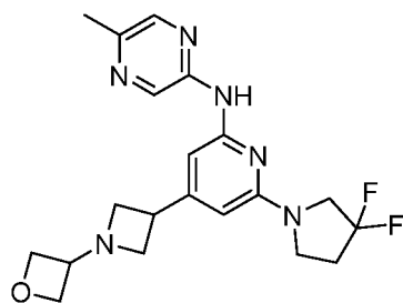
Compound 235
