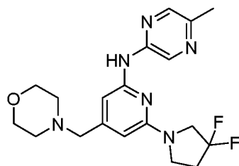
Compound 172
