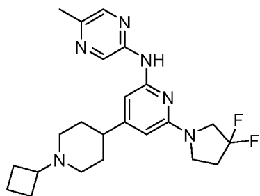
5 Compound 162
