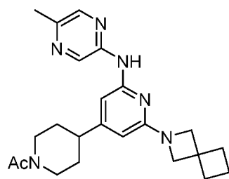
Compound 202
