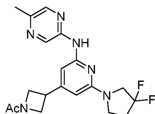
Compound 165
