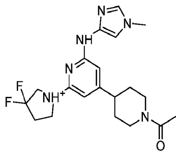
Compound 105
