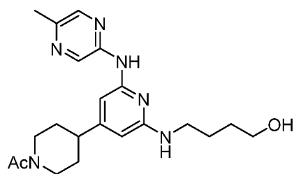
Compound 184
