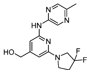
Compound 233
