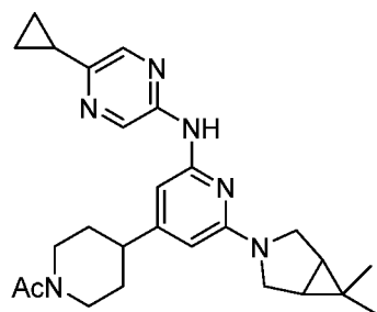
Compound 215
