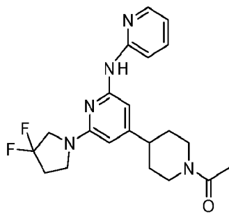
Compound 118
