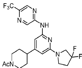
Compound 149
