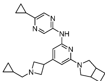
Compound 228
