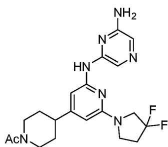
Compound 110
