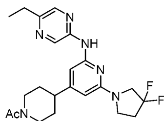
Compound 151
