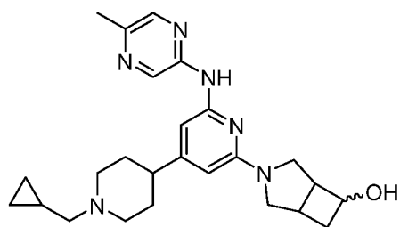
Compound 232
