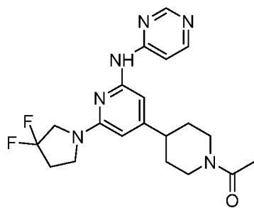
Compound 116
