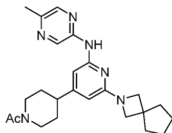
Compound 203
