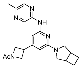
Compound 224
