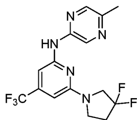
Compound 171
