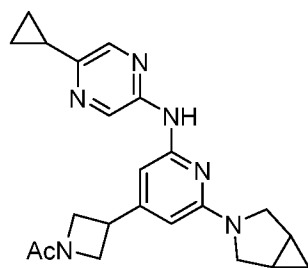
Compound 218
