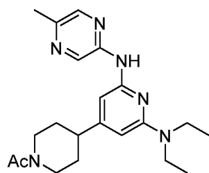
Compound 187
