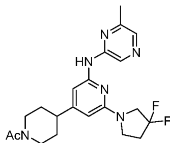
Compound 108
