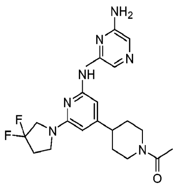
Compound 127
