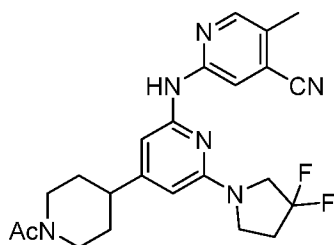
Compound 230
