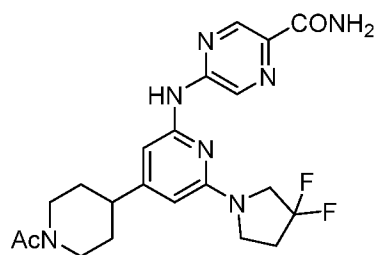
Compound 152
