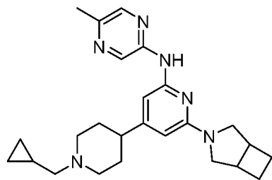
Compound 222
