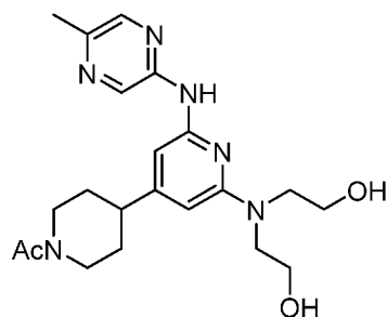
Compound 188
