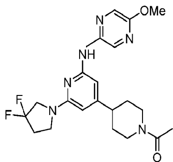
5 Compound 115
