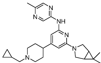
Compound 214
