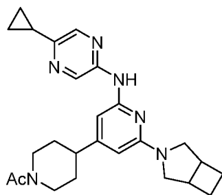
Compound 226
