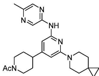
Compound 208
