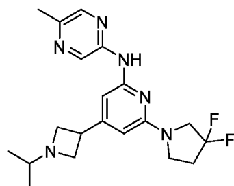
Compound 166
