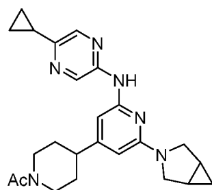
Compound 217
