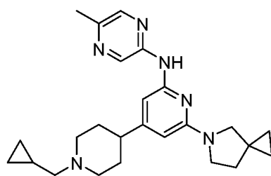
Compound 221
