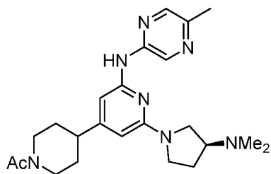
Compound 196
