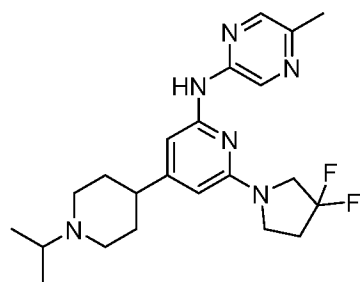
Compound 160
