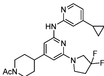
Compound 229
