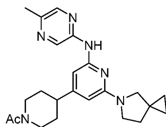
Compound 201
