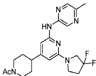
Compound 107
