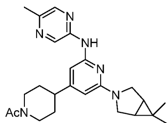
Compound 199
