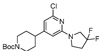
tert-butyl 4-(2-chloro-6-(3,3-difluoropyrrolidin-1-yl)pyridin-4-yl)piperidine-1-carboxylate
