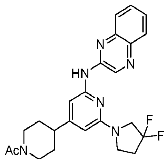
Compound 112
