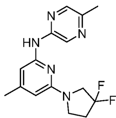
Compound 170
