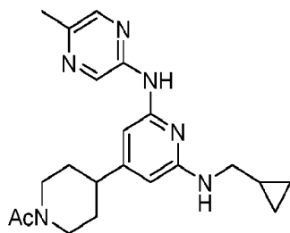
Compound 185
