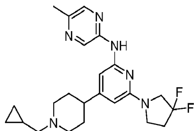
Compound 161
