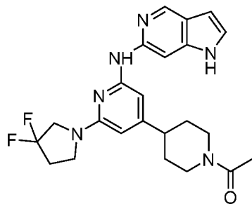
Compound 104
