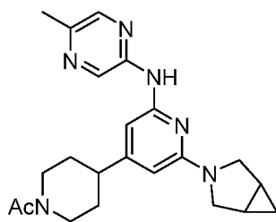
Compound 198
