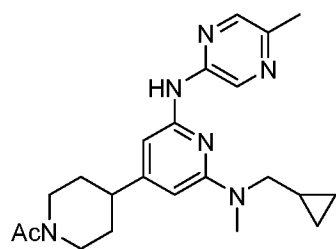
Compound 186
