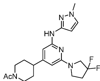
Compound 101
