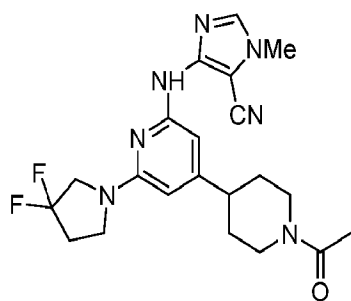
Compound 113
