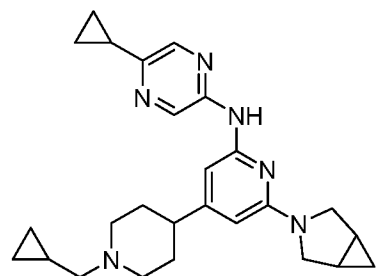
Compound 216
