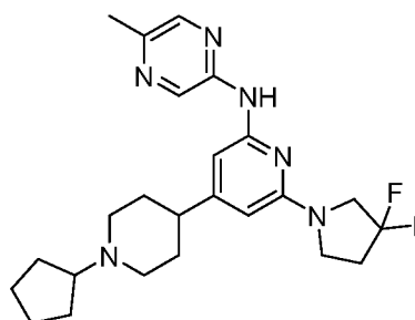
15 Compound 164
