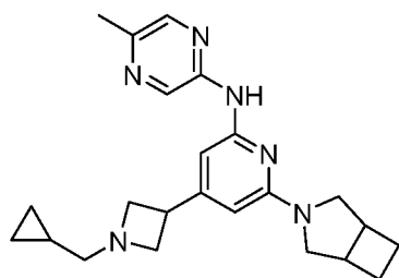
Compound 223
