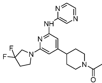
Compound 100
