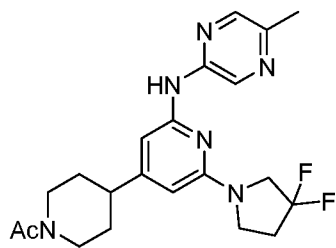
Compound 107
