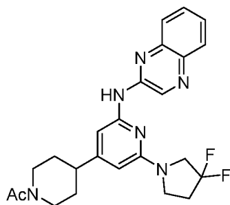
Compound 112
