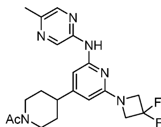
Compound 190
