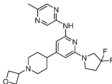
10 Compound 163
