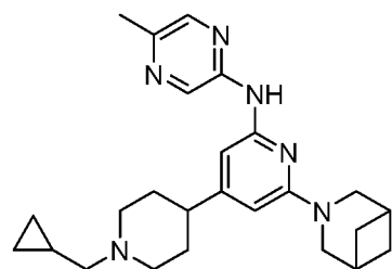
Compound 220
