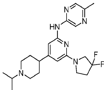
Compound 160
