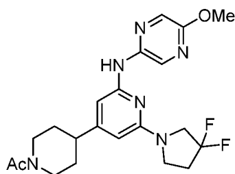
Compound 115
