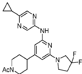
Compound 239
