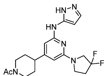
Compound 102
