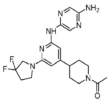
Compound 111
