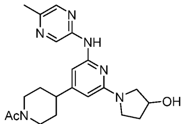
Compound 195
