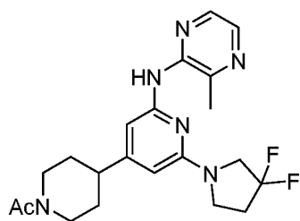
Compound 109
