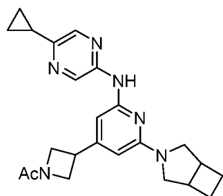
Compound 227
