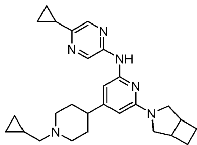
Compound 225
