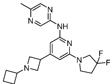
Compound 168
