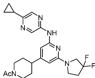
Compound 150
