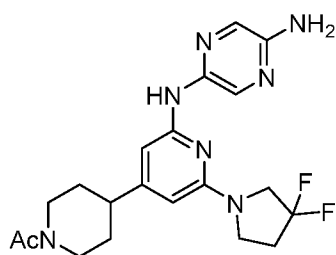
Compound 111
