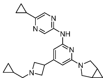
Compound 219
