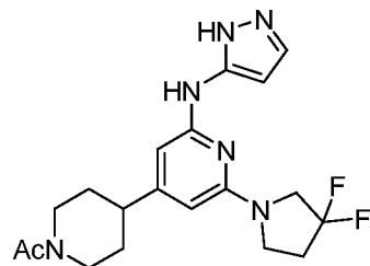
Compound 114
