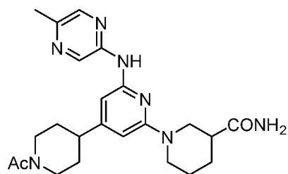
Compound 194
