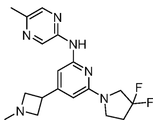
Compound 234
