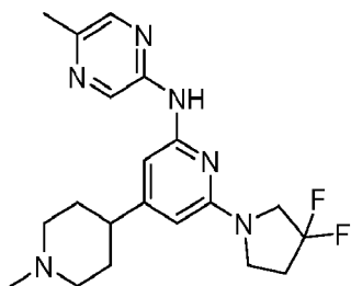
Compound 159
