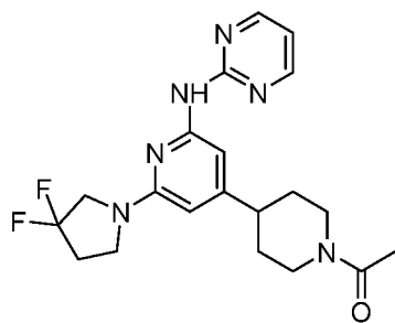
Compound 117
