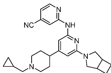
Compound 231
