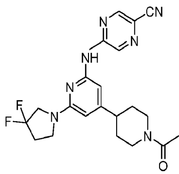
Compound 103
