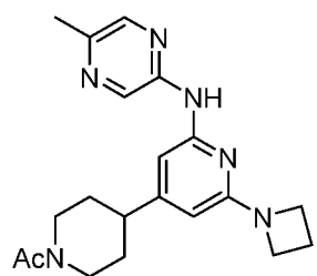
Compound 189
