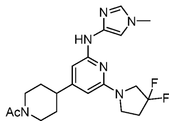
Compound 114
