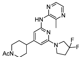
Compound 109
