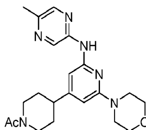
Compound 191
