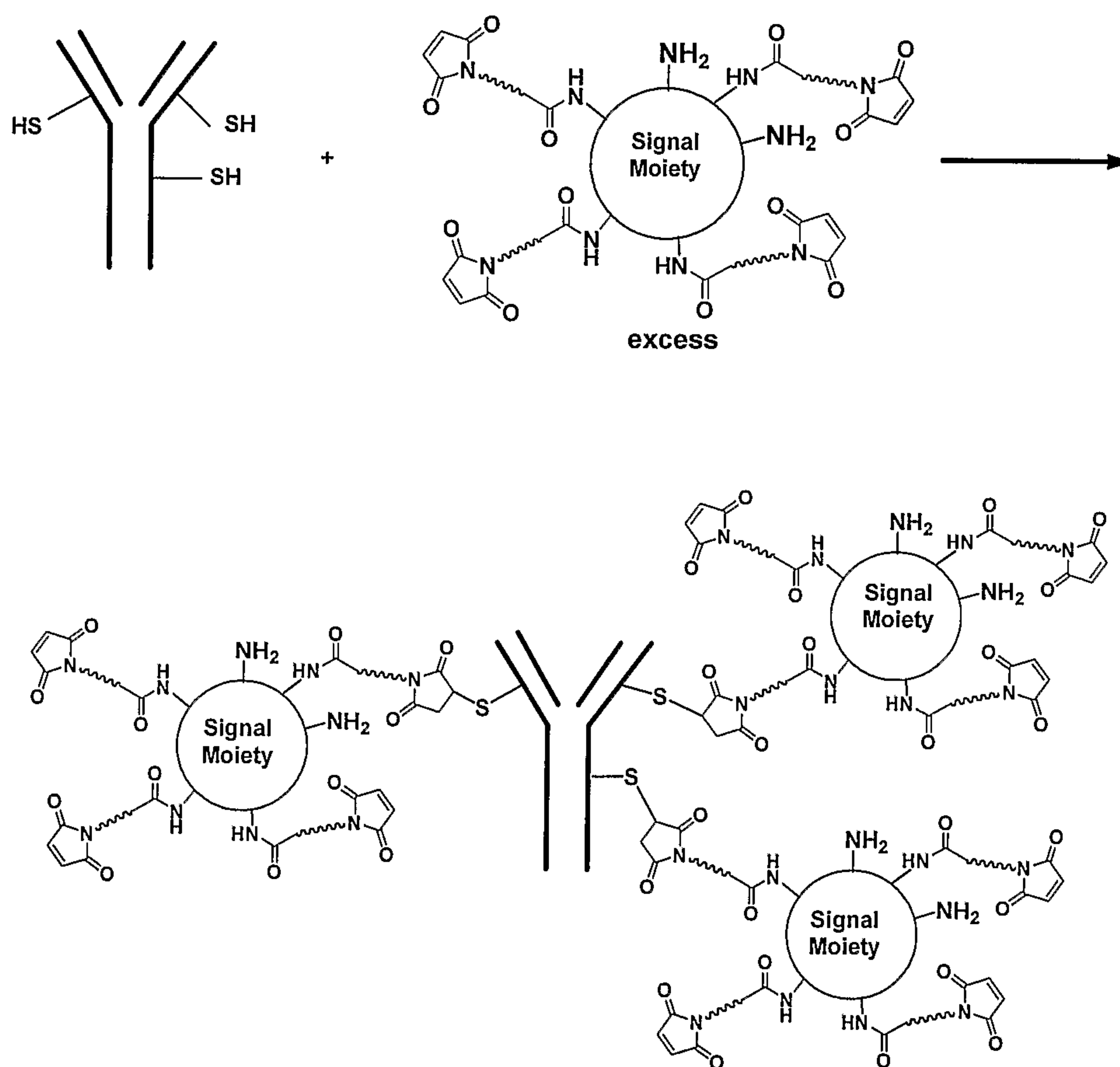
Scheme 3
