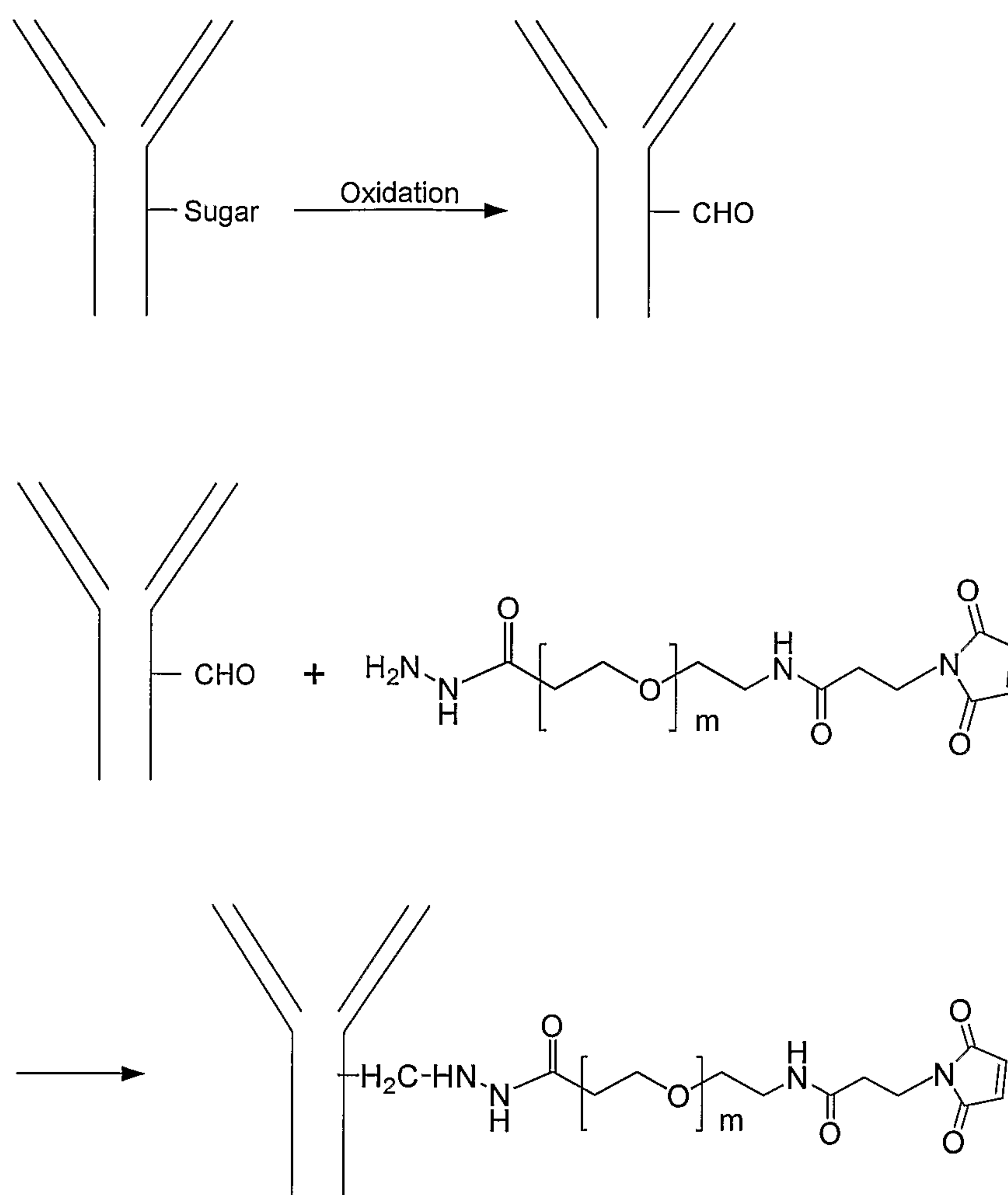
Scheme 4
