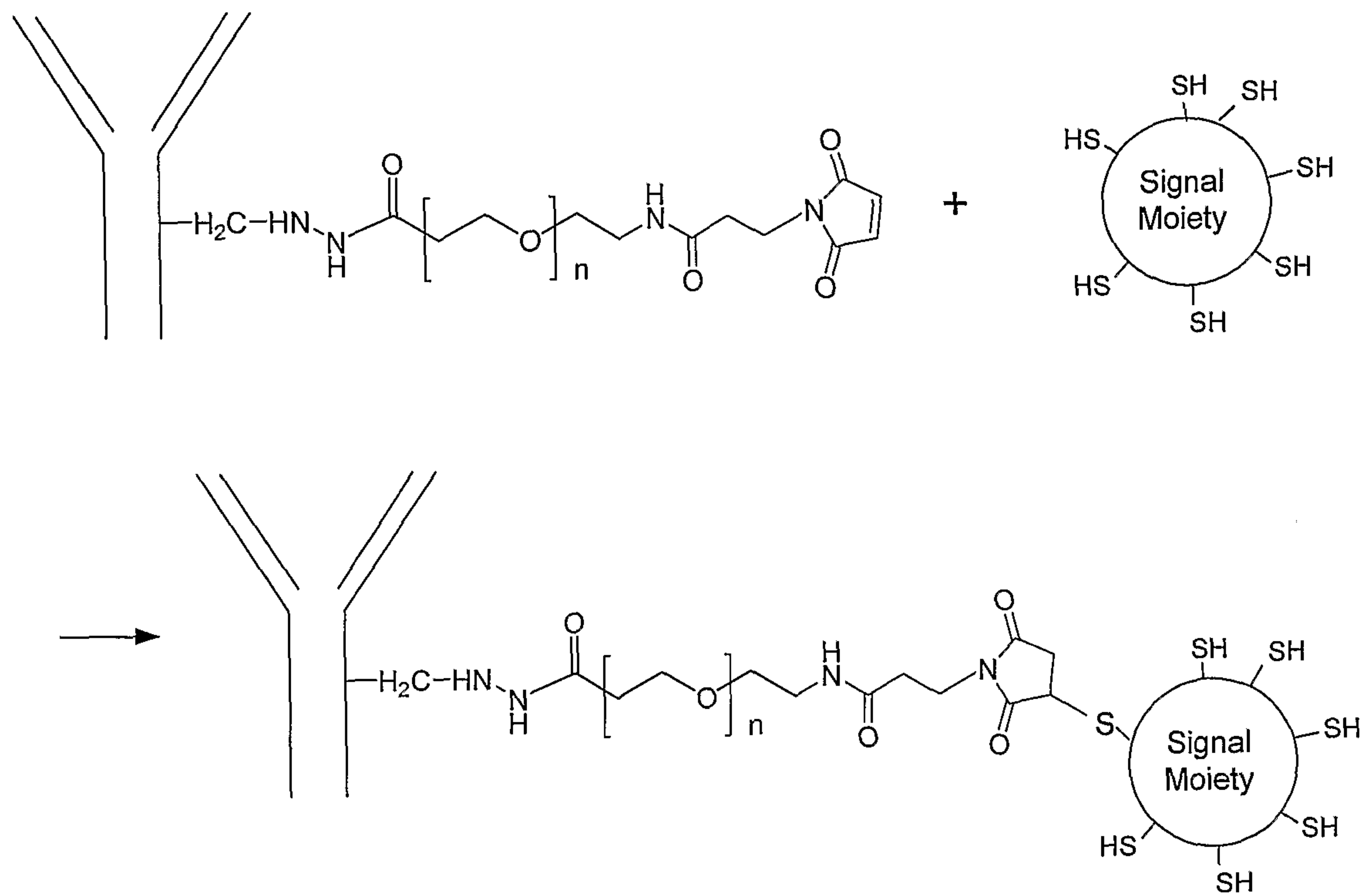
Scheme 5
