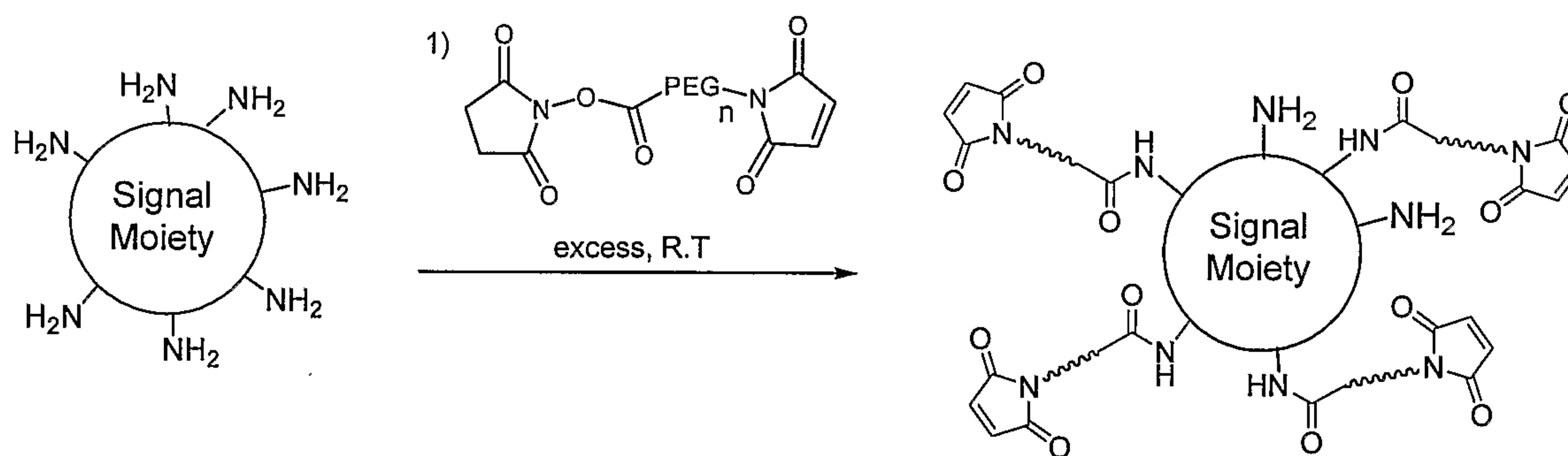
Scheme 1
