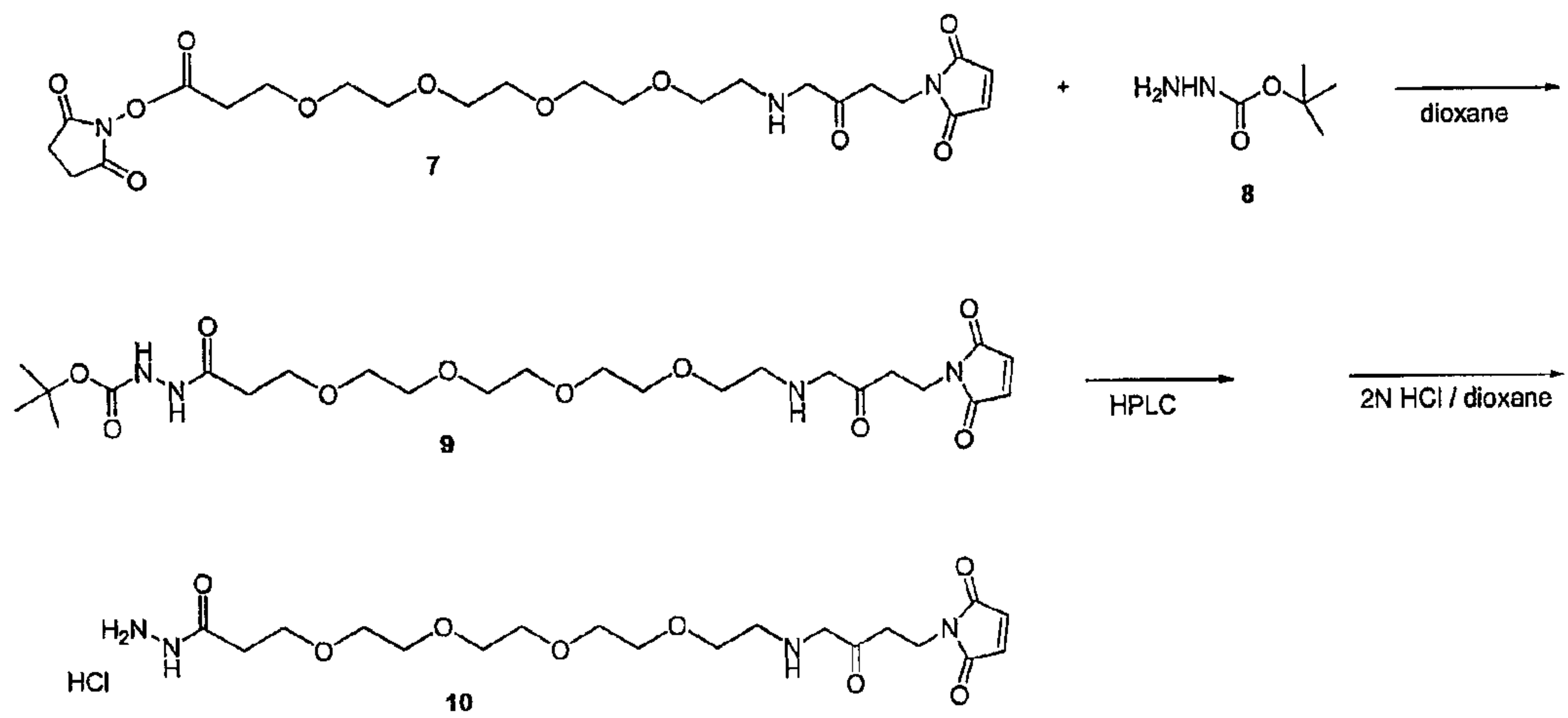
Scheme 7
