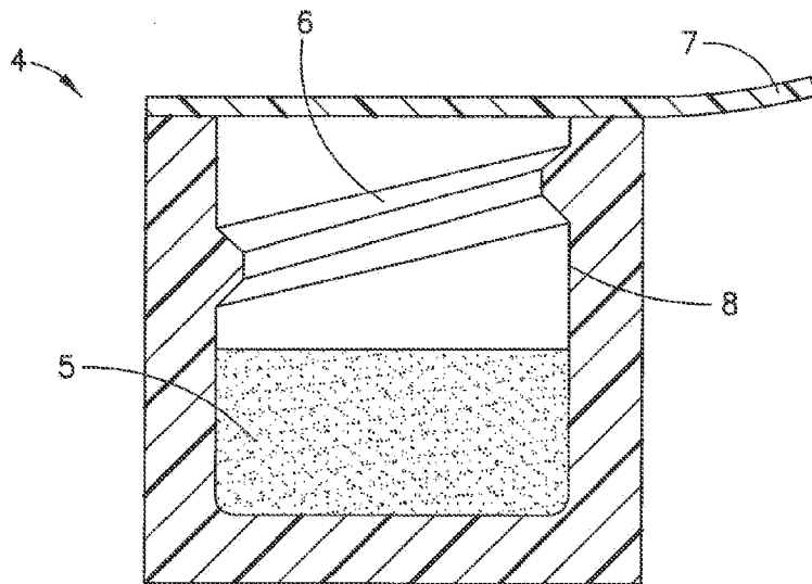
CONVENTIONAL FIG. 1B
