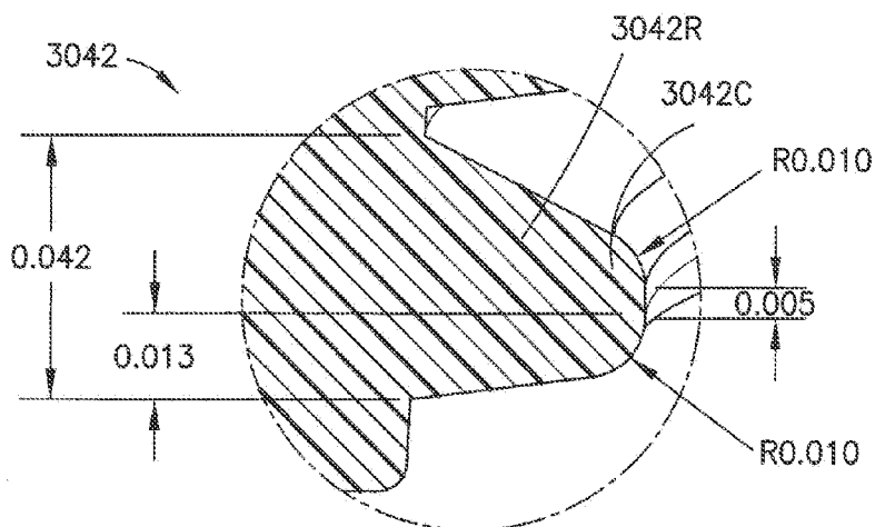
DETAIL A FIG. 24I
