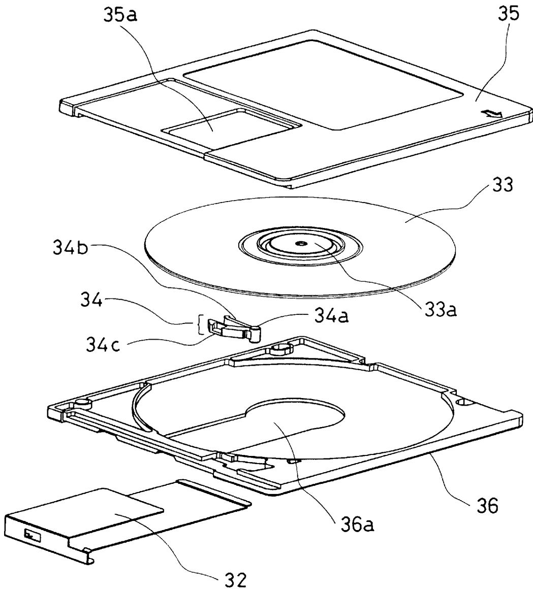
FIG. 10 PRIOR ART
