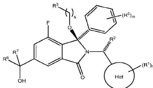
Diastereoisomer 1B
