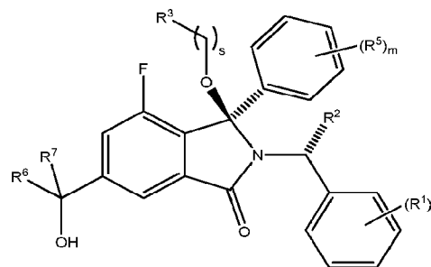
Diastereoisomer 1B
