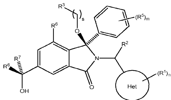
Diastereoisomer 2B
