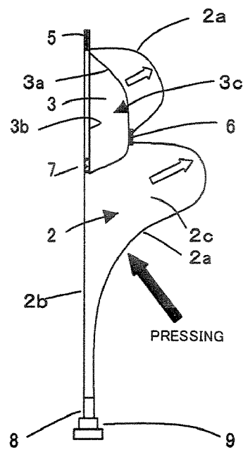
(c) X-X LINE CROSS-SECTION
