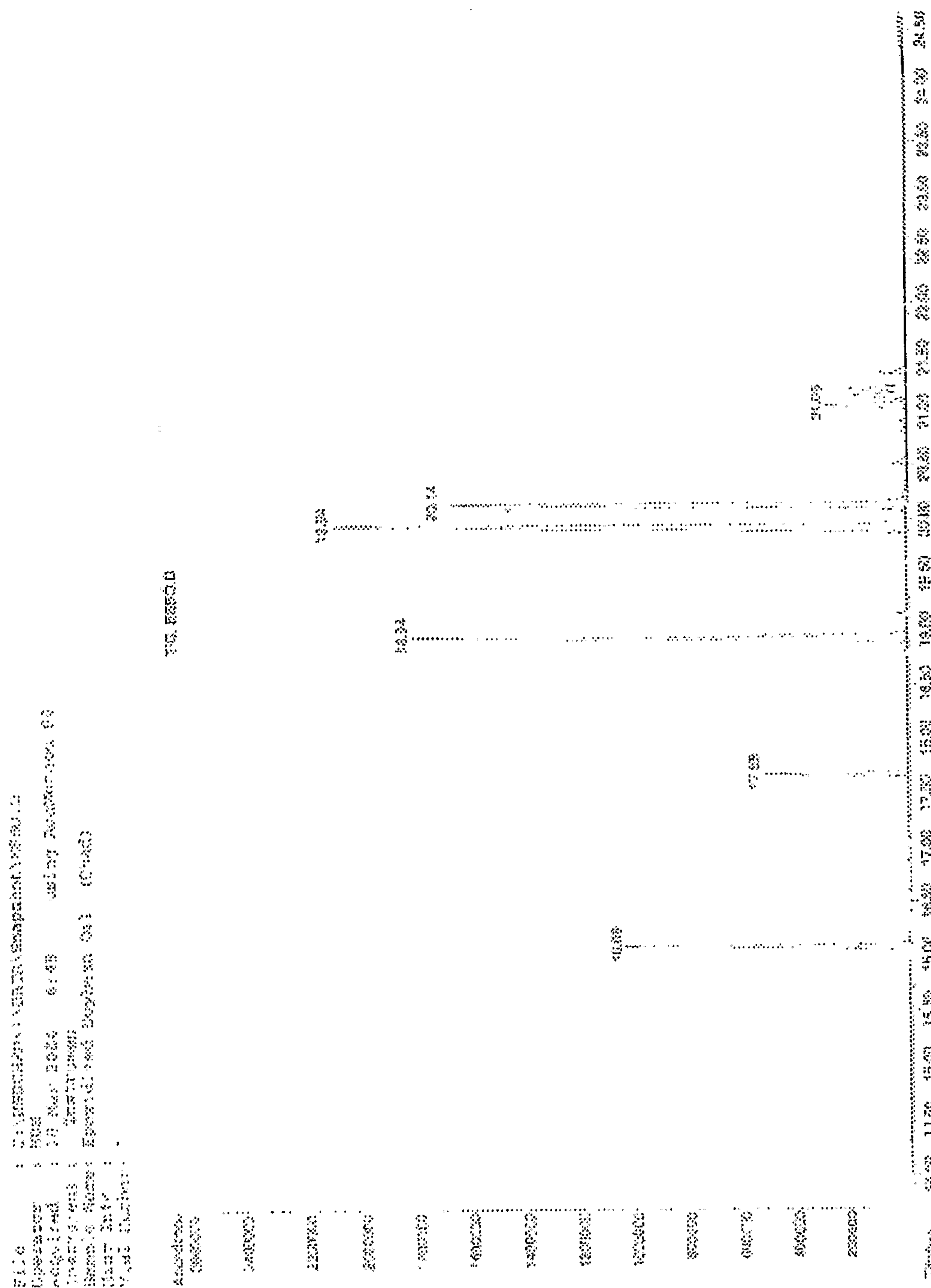
Figure 4 - GC/MS Trace of Epoxidized Soybean Oil Treated by Methanolysis
