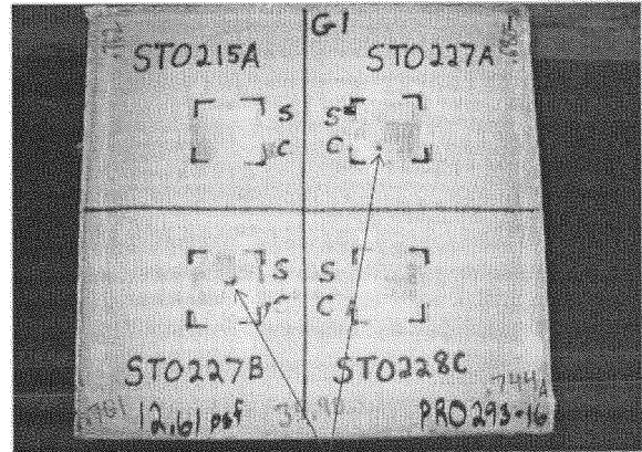
Back plate - Two (2) CP shots through the integrated batteries; no anomalous observations
