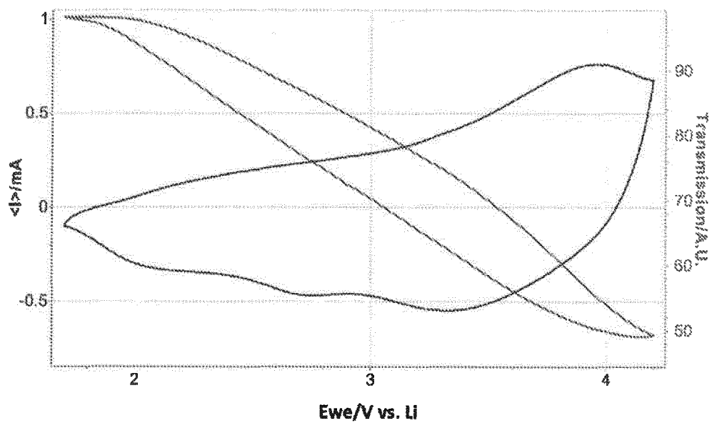
Figure 1 \text{LiNiZrVO}_x (~80 nm, CV, 50 th cycle)
