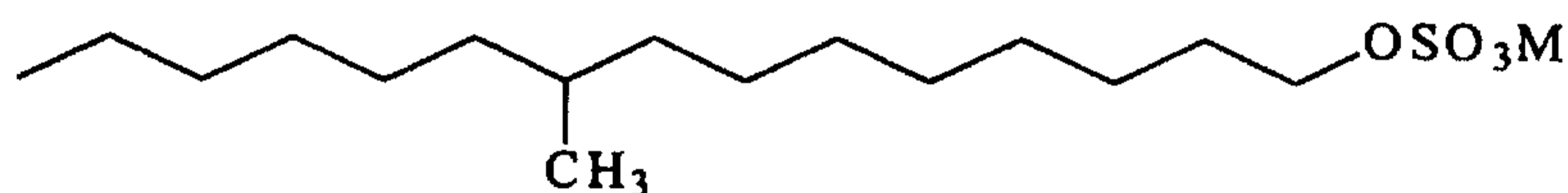
10-methylpentadecylsulfate having the formula
