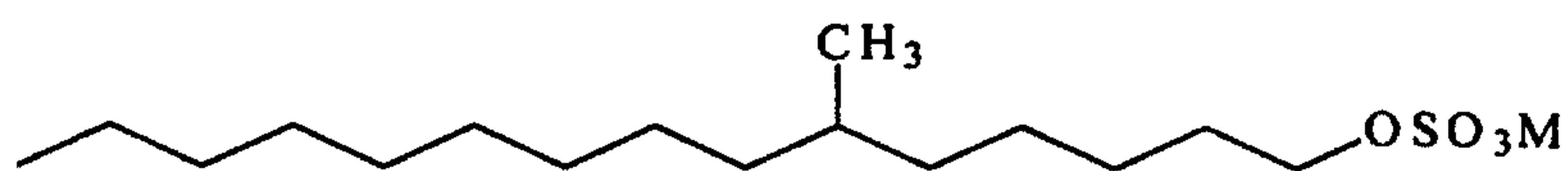
7-methylpentadecylsulfate having the formula
