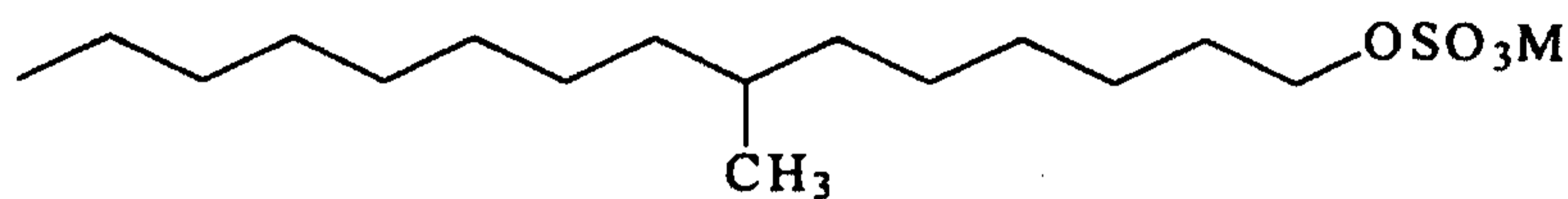
8-methylpentadecylsulfate having the formula
