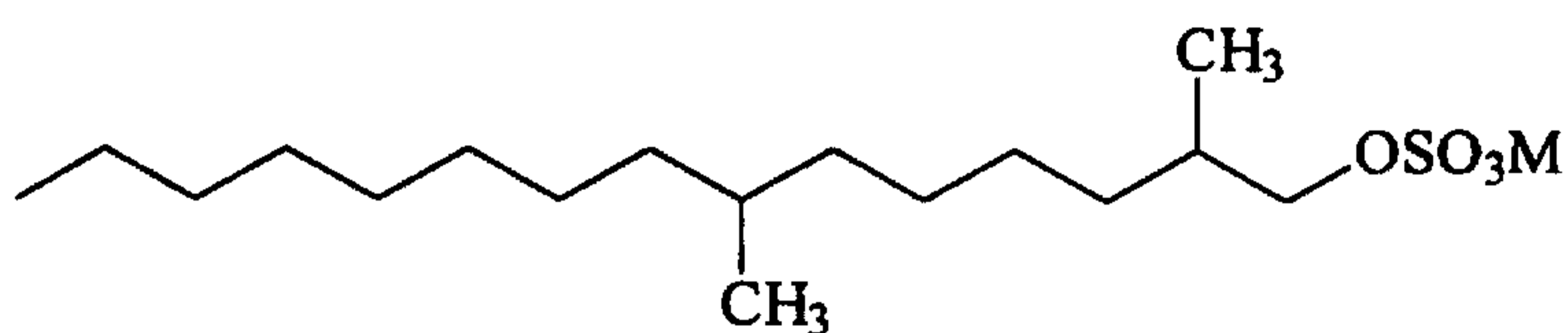
2,8-dimethylpentadecylsulfate having the formula
