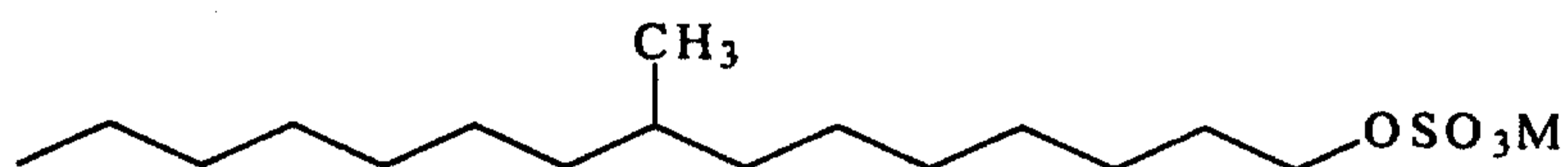
9-methylpentadecylsulfate having the formula
