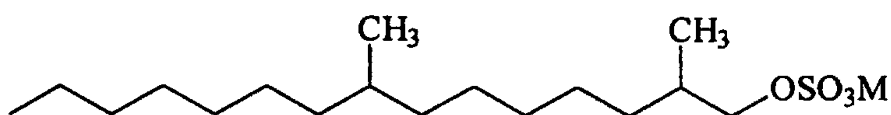
2,9-dimethylpentadecylsulfate having the formula
