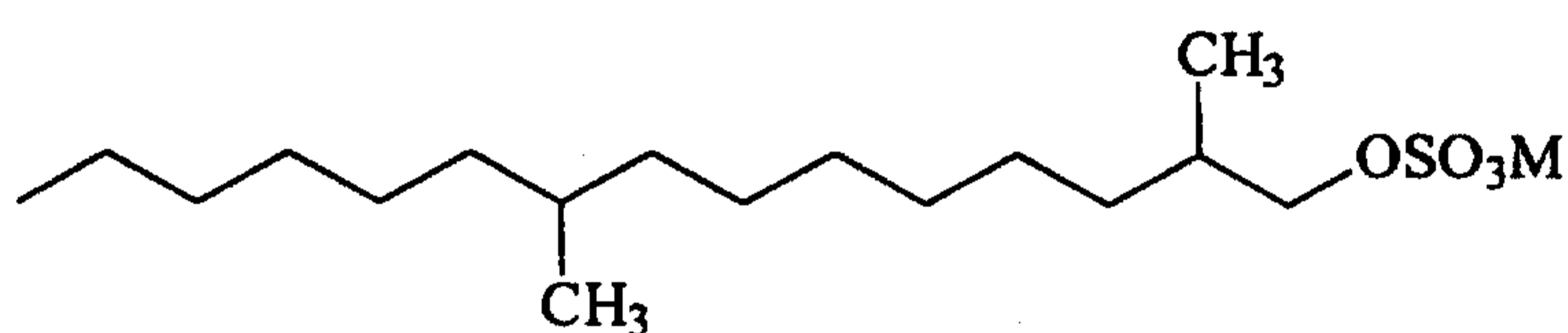
2,10-dimethylpentadecylsulfate having the formula
