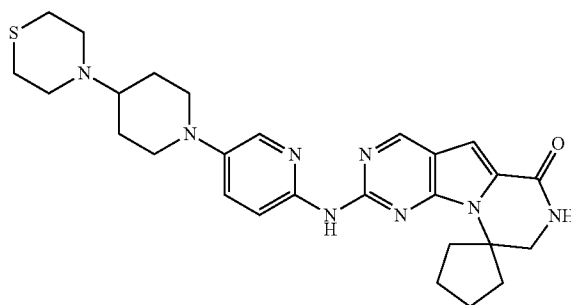
Compound 43
