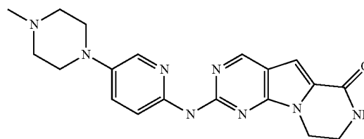
Compound 1
