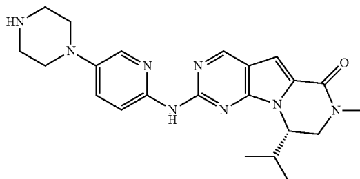
Compound 11
