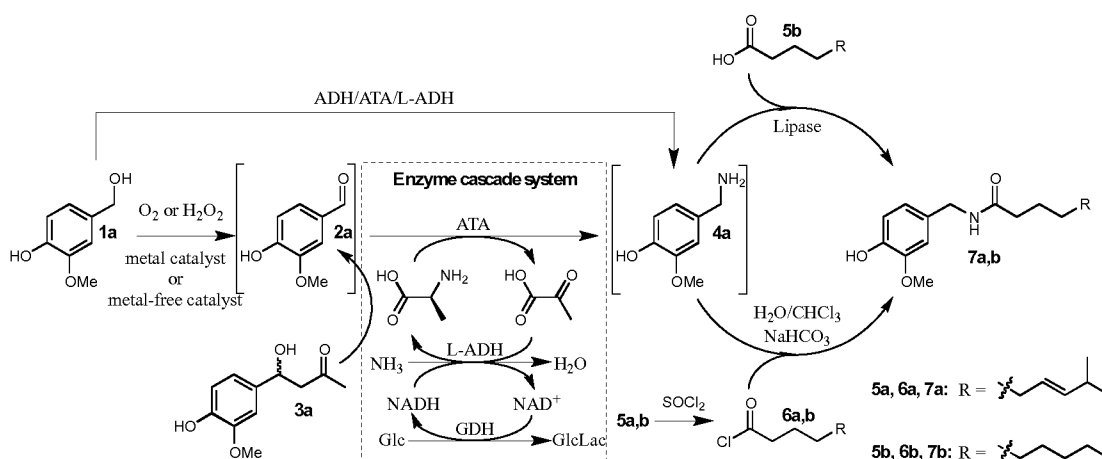
Scheme 2 – Conversion of vanillyl alcohol
