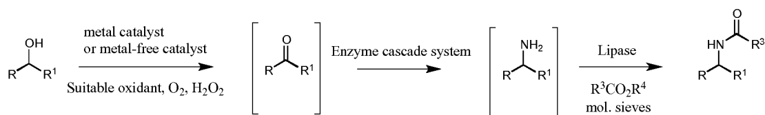
Scheme 1 – conversion of an alcohol
