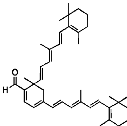
all- trans -retinal dimer
