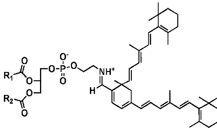
all- trans -retinal dimer-phosphatidylethanolamine
