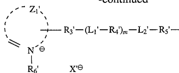
Formula (H2)
