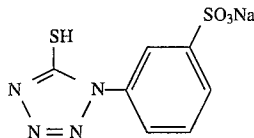
Triazine compound (c)
