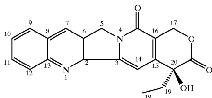
Figure 1-Camptothecin
