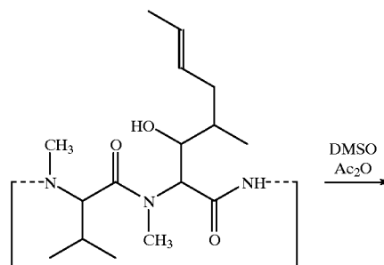
Cyclosporin A
