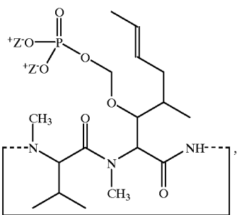
Cyclosporin A
