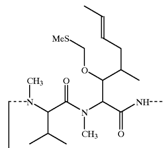
Cyclosporin A
