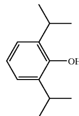
Propofol (2,6-diisopropylphenol)
