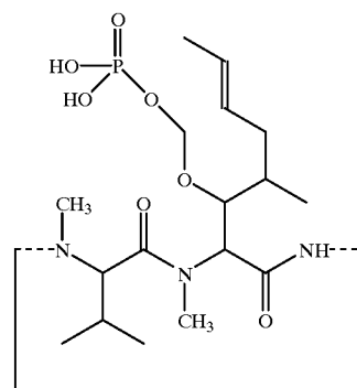
Cyclosporin A
