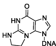
N 2 ,3-ethano-guanine
