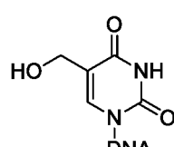
5-hydroxymethyl-uracil
