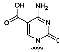
5-carboxy-dC
