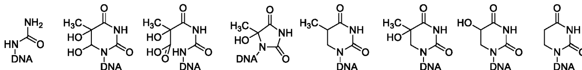
urea thymine glycol ( cis & trans ) methyl tartonyl urea 5-hydroxy-5- methylhydantoin 5,6-dihydro thymine 5-hydroxy-6- hydrothymine 5-hydroxy-6- hydouracil 5,6- dihydro- uracil
