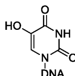
5-hydroxy- uracil
