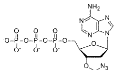
3'-O-azidomethyl-dATP:
