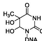
thymine glycol ( cis & trans )
