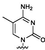
5-methyl-dC
