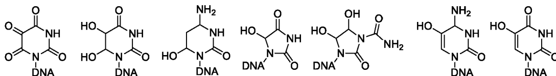
alloxan uracil glycol ( cis & trans ) 6-hydroxy-5,6- dihydrocytosine 5-hydroxy hydantoin trans -1-carbamoyl- 2-oxo-4,5-dihydroxy- imidazolidine 5-hydroxy- cytosine 5-hydroxy- uracil
