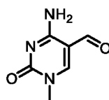
5-formylcytosine
