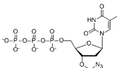
3'-O-azidomethyl-dATP:
