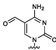
5-formyl-dC
