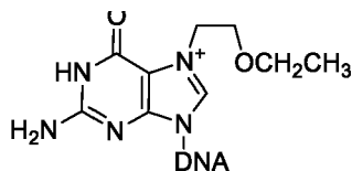
7-(2-ethoxyethyl)- guanine
