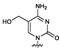
5-hydroxymethyl-dC
